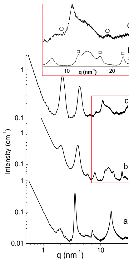
Fig. 2 SAXS profiles of a) M1, b) M1-Pd(II) and c) M1-Pt(IV). The squares and the black rings in the inset correspond respectively to the supplemental structure peaks at wide angles of b) M1-Pd(II) and c) M1-Pt(IV).
