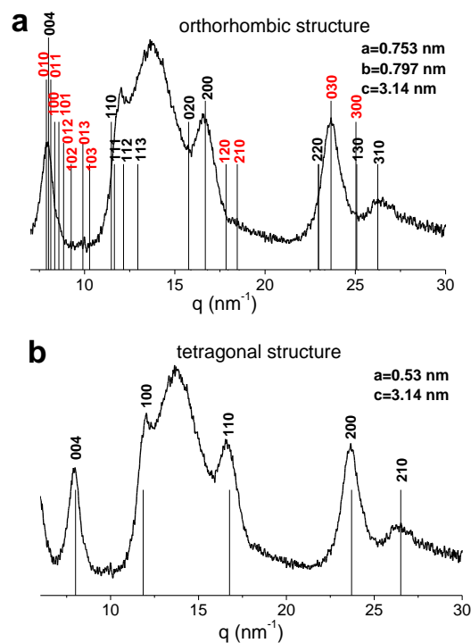
Fig. 4 Calculation of a) the orthorhombic structure and b) the structure tetragonal structure compared to the M1-Pd(II) SAXS profile. The red indexes exhibit Bragg reflections whose indexes h and k are of different parity in the case of the orthorhombic structure.
