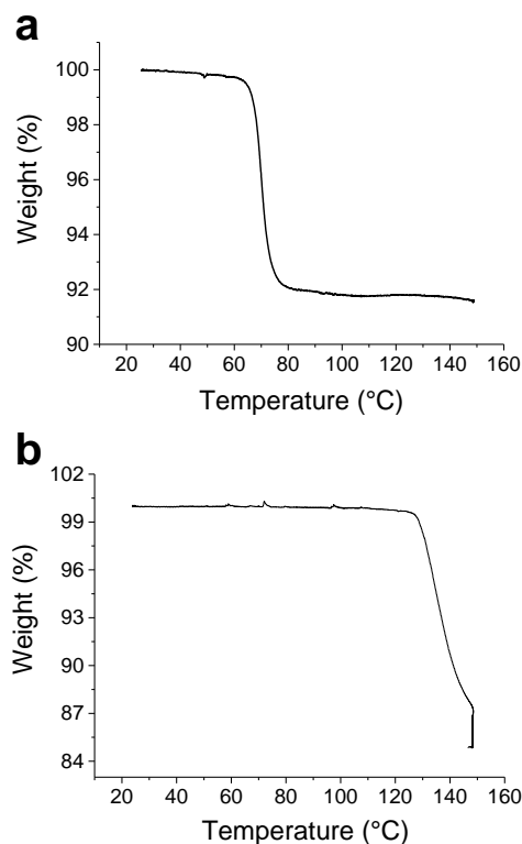
Fig. 8 In situ thermal reduction analysis of a) M1-Pd(II) and b) M1-Pt(IV).
