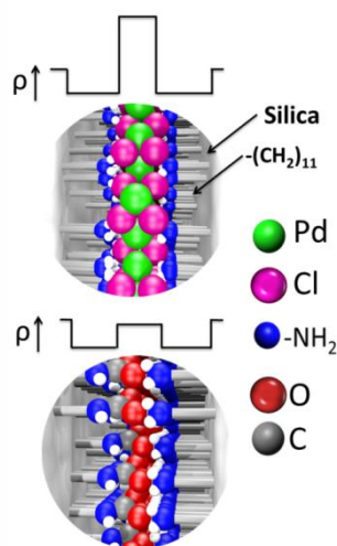
Fig. 3 Schematic representation of the lamellar structure with carbon dioxide or metallic salt at the interface between two organosilica bilayers. The value of the electronic density \rho of each part of the lamellar structure is also represented. Inset: schematic representation of the crystalline monolayer phase of \text{PdCl}_2 (composed of \text{PdCl}_4^{2-} units) at the interface between two organosilica bilayers in the M1-Pd(II) material.
