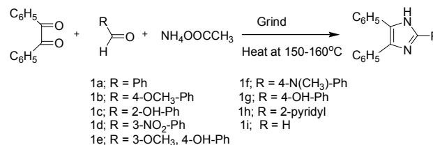
Scheme 1 R-I synthesis of tri-substituted imidazoles (1a-1i)
