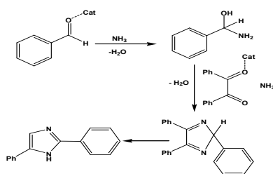
Scheme 4 Mechanism of the R-I synthesis
