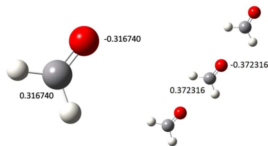
Fig. 5 Minimum energy models with partial charges.
