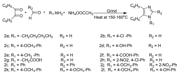
Scheme 2 R-I synthesis of tetra-substituted imidazoles (2a-2l)
