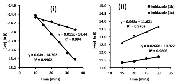
Fig. 2 (–ve)/(+ve) \ln(I) vs time(mins) of [i] benzil during formation of imidazoles (1b) and (1c); [ii] rate curve of the product imidazoles (1b) and (1c) formation; I = Peak A.
