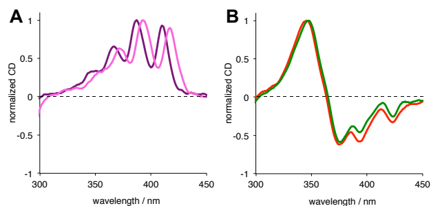
Figure 4. Circular dichroism spectra of 500 \mu\text{M} AmB in ILs; A : [\text{C}_4\text{-mim}]\text{Br} (pink), [\text{C}_4\text{-mim}]\text{CF}_3\text{CO}_2 (purple); B [\text{C}_4\text{-mim}]\text{NTf}_2 (red), [\text{C}_4\text{-mim}]\text{PF}_6 (green).
