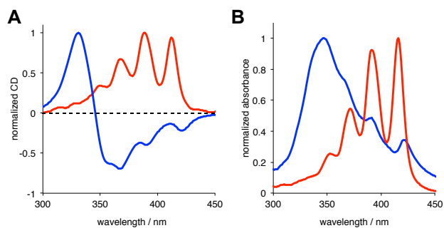
Figure 2. Circular dichroism (A) and absorption (B) spectra of 500 \mu\text{M} AmB in water (blue) and DMSO (red).
