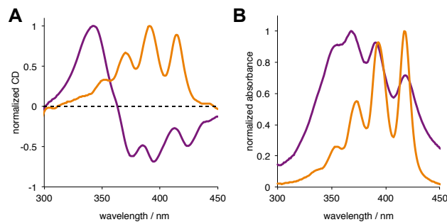
Figure 3. Circular dichroism (A) and absorption (B) spectra of 500 \mu\text{M} AmB in [C 4 -mim]BF 4 (purple) and [C 4 -mim]NO 3 (orange).
