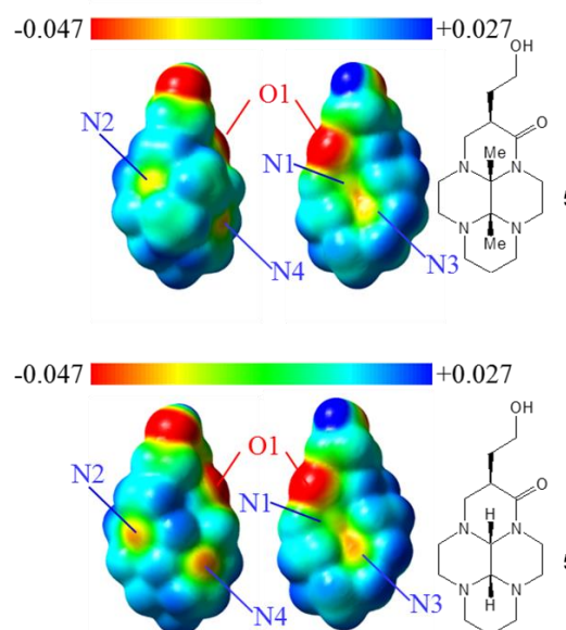
Fig. 4 Computed TPSSh/6-311G(d,p) electrostatic potentials (hartree) of 5 (bottom) and 5' (top) on the molecular surfaces defined by the 0.001 \text{ electrons}\cdot\text{bohr}^{-3} contour of the electronic density. Convex sides are represented on the left and concave ones on the right.
