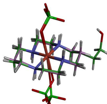
Fig. 7 Superposition of the X-ray crystal structures of [\text{Cu}(\text{cyclam-EtOH})](\text{ClO}_4)_2 15 (green) and [\text{Cu}(\text{cyclam})](\text{ClO}_4)_2 25 (purple).
