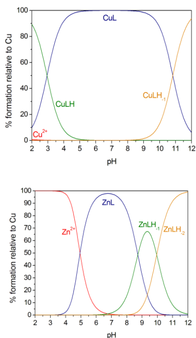
Fig. 6 Copper(II) and zinc(II) speciation diagrams in the presence of Cyclam-EtOH. [\text{M}^{2+}]_{\text{tot}} = [\text{L}]_{\text{tot}} = 10^{-3} M.
