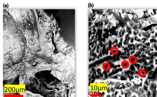
Fig. 3 SEM images of pure/dried soya nugget (a,b)
