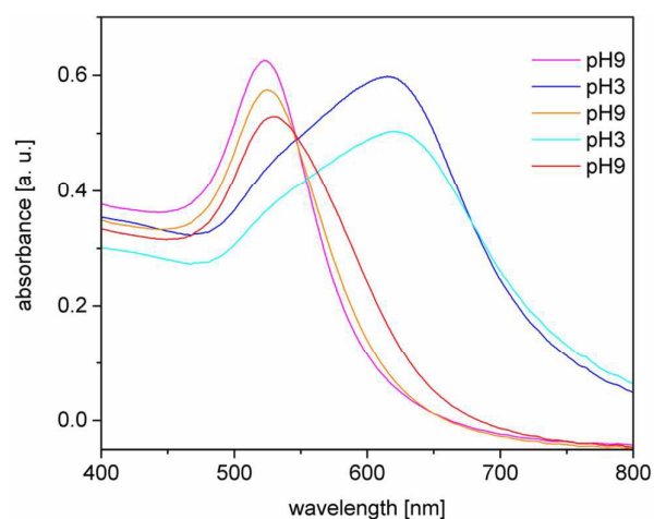
Fig. 2: UV-vis spectra of pH dependent agglomeration of irradiated c /DA-COOH-AuNP, while alternately adding acids (blue) and bases (red) starting with pH 9 (pink).
