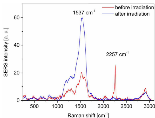
Fig. 3: SERS spectra of DA-COOH-AuNP before (red) and after (blue) irradiation with UV-light (254 nm) for 15 min. The signal at 2257 \text{cm}^{-1} is assigned to stretching vibrations of the carbon-carbon triple bond. The signals in the region of 1000 – 1600 \text{cm}^{-1} are attributed to the stretching vibrations of carbon-carbon double bonds. The signal broadening is attributed to different polymer lengths.
