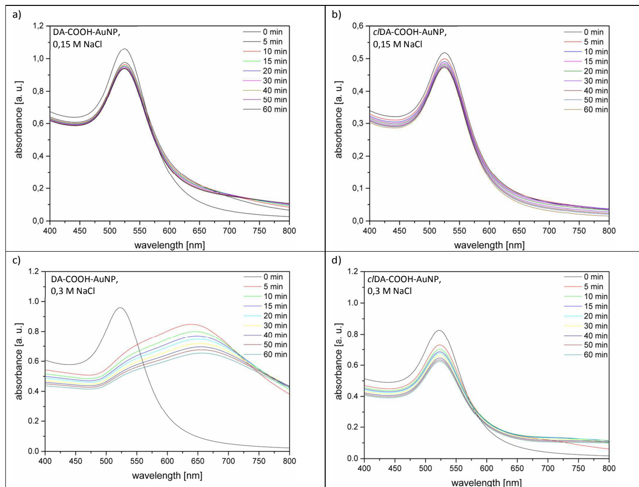
Fig. 4: UV-vis spectra of a) non-irradiated DA-COOH-AuNP, 0.15 M NaCl, b) irradiated c /DA-COOH-AuNP, 0.15 M, c) non-irradiated DA-COOH-AuNP, 0.3 M NaCl and d) irradiated c /DA-COOH-AuNP, 0.3 M NaCl before (black graph) and after addition of NaCl solution at different points in time after addition (5 min, 10 min, 15 min....60 min.).
