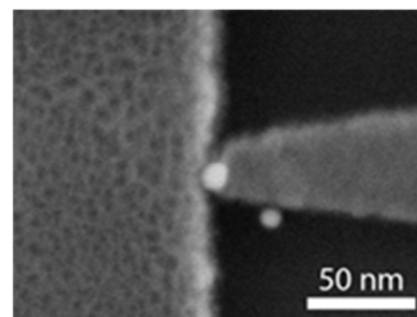
Fig. 7: Exemplarily SEM image of the setup used to electrically characterize an individual c /DA-COOH-AuNP immobilized in between a Pt- and a AuPd-electrode comprising a gap of about 13 nm.
