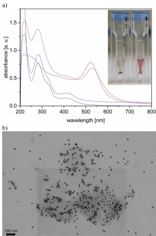
Fig. 5: a) UV-vis spectra of non-irradiated DA-COOH-AuNP (blue solid line) and irradiated c /DA-COOH-AuNP (red solid line) after incubation with DTT at 60°C. For reference purposes the UV-vis spectrum of non-irradiated DA-COOH-AuNP (blue dashed line) and irradiated c /DA-COOH-AuNP (red dashed line) without DTT, respectively, as well as the UV-vis spectrum of DTT (black solid line) are also displayed. Inset: photography showing solutions of non-irradiated DA-COOH-AuNP (left) and irradiated c /DA-COOH-AuNP (right) after addition of DTT. b) SEM-T image of irradiated c /DA-COOH-AuNP after incubation with DTT at 60°C. Mean particle size 13.4 nm \pm 1.2 nm (156 Particles counted)
