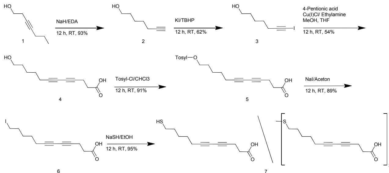
Scheme 2: Preparation of the ligand DA-COOH.
