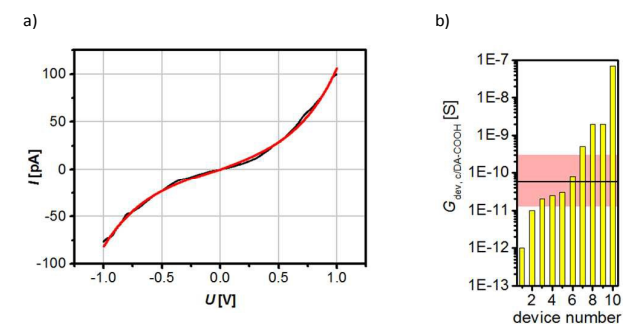
Figure 8: a) Current/voltage-characteristic: the black curve corresponds to the average of several measured cycles and the red curve to the Simmons fit. b) Histogram of the conductance values of 10 c /DA-COOH-AuNP devices at 1 V. The horizontal black line shows the median and the light red bar marks values from 1/5 times the median to 5 times the median.
