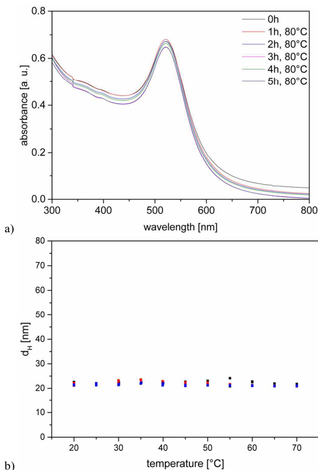
Fig. 6: a) UV-vis spectra recorded on a dispersion of c /DA-COOH-AuNP in buffer solution (pH 8) heated at 80 °C for 5h. b) Evolution of the hydrodynamic radii ( d_H ) of c /DA-COOH-AuNP during 3 heating and cooling cycles switching repeatedly between 20 °C and 70 °C forth and back.
