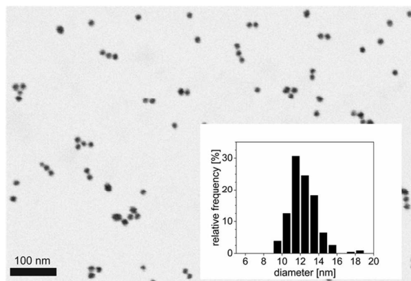
Fig. 1: Representative SEM-T Image of c /DA-COOH-AuNP with histogram (inset). The particle size was determined to 12.3 nm \pm 1.4 nm (based on 231 AuNP counted).
