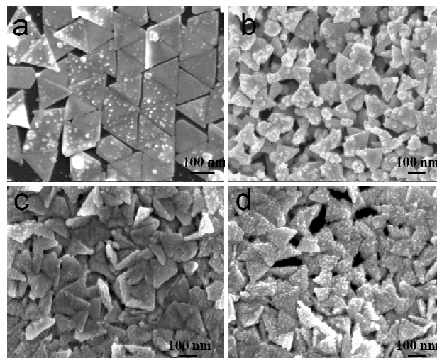
Fig. 3 Representative FE-SEM images of tiny Ag nanoparticles grown on triangular Au nanoplates at different volume ratio's of growth solution: 0.2:0.1 ml (a), 0.5:0.25 ml (b), 1:0.5 ml (c), and 2:1 ml (d), respectively. The scale bars represent 100 nm.
