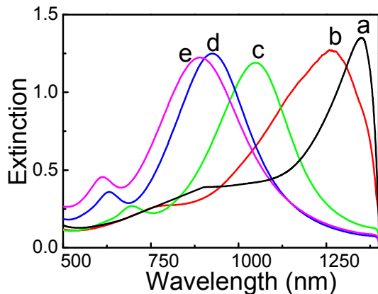
Fig. 2 UV-vis-NIR absorption spectra of triangular Au nanoplates obtained before (a) and after in different volumes of \text{AgNO}_3 :AA growth solution in the respective tubes 0.2:0.1 ml (b), 0.5:0.25 ml (c), 1:0.5 ml (d), and 2:1 ml (e) for growing tiny AgNPs.
