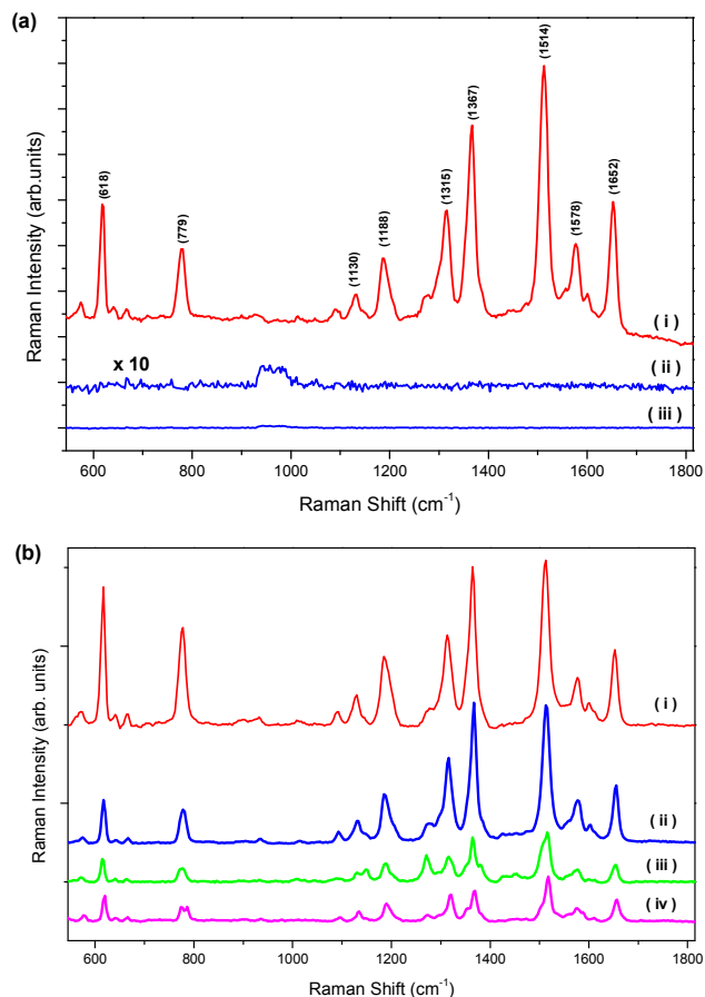
Fig. 8 (a) i. SER spectrum of 1\text{ }\mu\text{M} R6G on branched gold NPs grown on Si-substrate. ii. Raman spectrum of 1\text{ mM} R6G on Si-substrate (Multiplied by 10). iii. Raman spectrum of 1\text{ mM} R6G on Si substrate (b) SER spectra of i. 1\text{ }\mu\text{M} R6G, ii. 0.1\text{ }\mu\text{M} R6G, iii. 0.01\text{ }\mu\text{M} ( 10\text{ nM} ) R6G and iv. 0.001\text{ }\mu\text{M} ( 1\text{ nM} ) R6G on branched gold NPs grown on Si-substrate.
