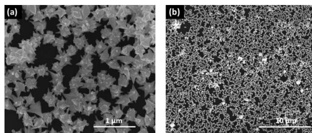
Fig. 3 SEM images (at different magnifications) of branched gold nanoparticles on Si-substrates have shown with (a) 1 \mu m and (b) 10 \mu m scales.
