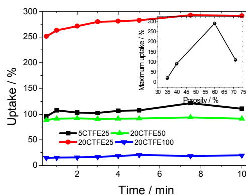
Fig. 4 Electrolyte uptake value as a function of time for the PVDF-CTFE separator samples
