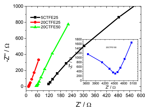
Fig. 6 Nyquist plots for the PVDF-CTFE separator samples.
