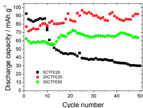
Fig. 10 Cycling performance of \text{C-LiFePO}_4 cathodic half cells containing the different PVDF-CTFE separator membranes at 2C.
