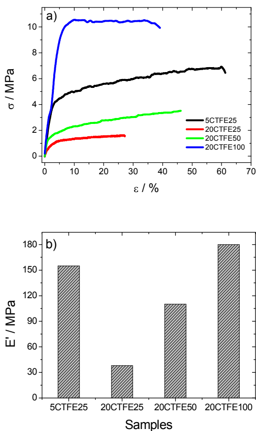
Fig. 5 a) Stress-strain curves and b) Young's modulus ( E' ) for the PVDF-CTFE separator samples.
