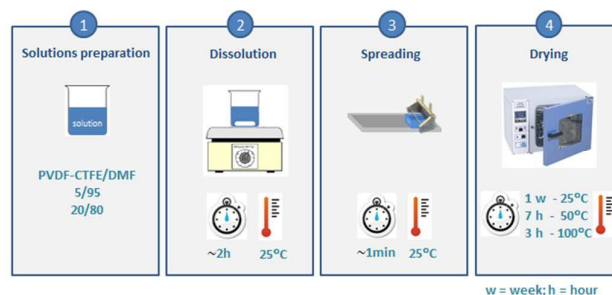
Fig. 1 Experimental procedure for the PVDF-CTFE membrane preparation.
