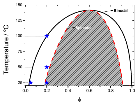
Fig. 2 Phase diagram of the binary PVDF-CTFE/DMF system, after 29 .
