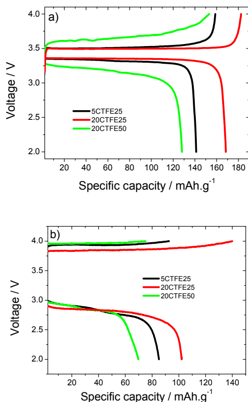
Fig. 9 Charge-discharge profiles for the PVDF-CTFE separator membranes at a) C/10 and b) 2C.
