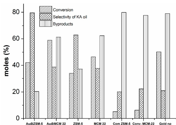
Figure 4. Conversion of cyclohexane and selectivity towards KA-oil for different catalyst. Amount of gold in case of control experiment was higher (1000 times) than in case of Au@ZSM-5 and Au@MCM-22.
