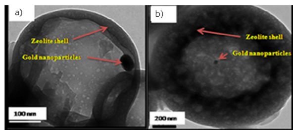
Figure 3. TEM images of spent a) Au@ZSM-5, b) Au@MCM-22 after oxidation of cyclohexane.
