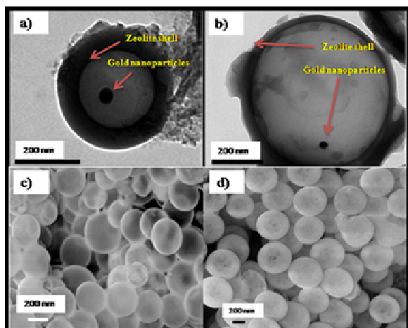
Figure 1. TEM images of a) Au@ZSM-5, b) Au@MCM-22. SEM images of c) Au@ZSM-5, d) Au@MCM-22 showing gold nanoparticle encapsulated inside zeolite shell.
