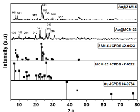
Figure 2. XRD analysis of Au@ZSM-5 and Au@MCM-22.
