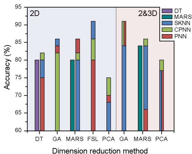
Figure 5. Accuracy of models obtained using different classification and dimension reduction techniques. The dimension reduction techniques are arranged by ascending number of descriptors.
