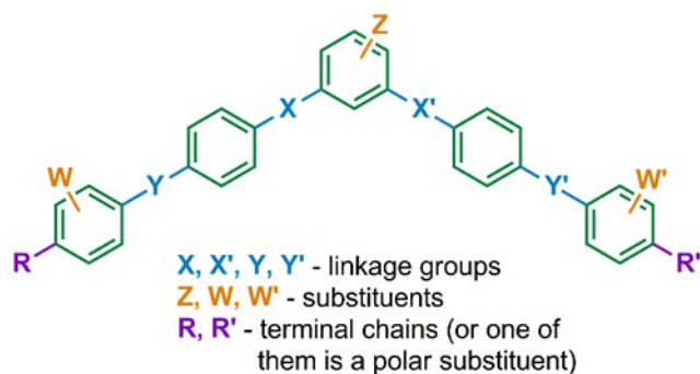
Figure 1. Schematic representation of the modelled five-ring bent-core system
