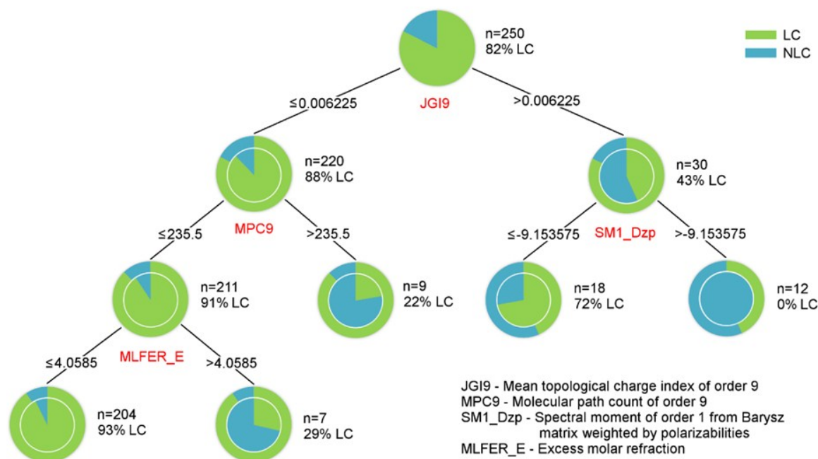
Figure 3. The decision tree model obtained for the classification of LCs. The outer ring of each node presents the “purity” of the parent node. The number of compounds in a node ( n ) and ratio of LCs is displayed near the corresponding node. The descriptors and their splitting values are presented between two levels.
