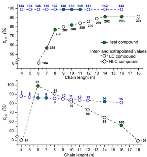
Figure 8. The p_{LC} trend in a homologous series as the number of carbons ( n ) in the terminal chain is increased.
