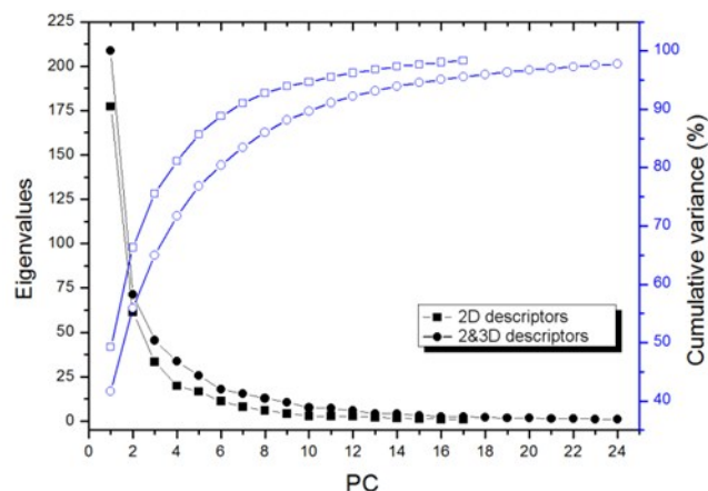
Figure 4. PCA components with eigenvalues and variance
