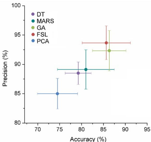
Figure 6. The average performance of classifiers created with descriptors selected by different techniques. The lines represent standard deviation. The number of DT and MARS based models is 4 and 8, respectively, while the number of GA, FSL and PCA models is the same, 6 of each.
