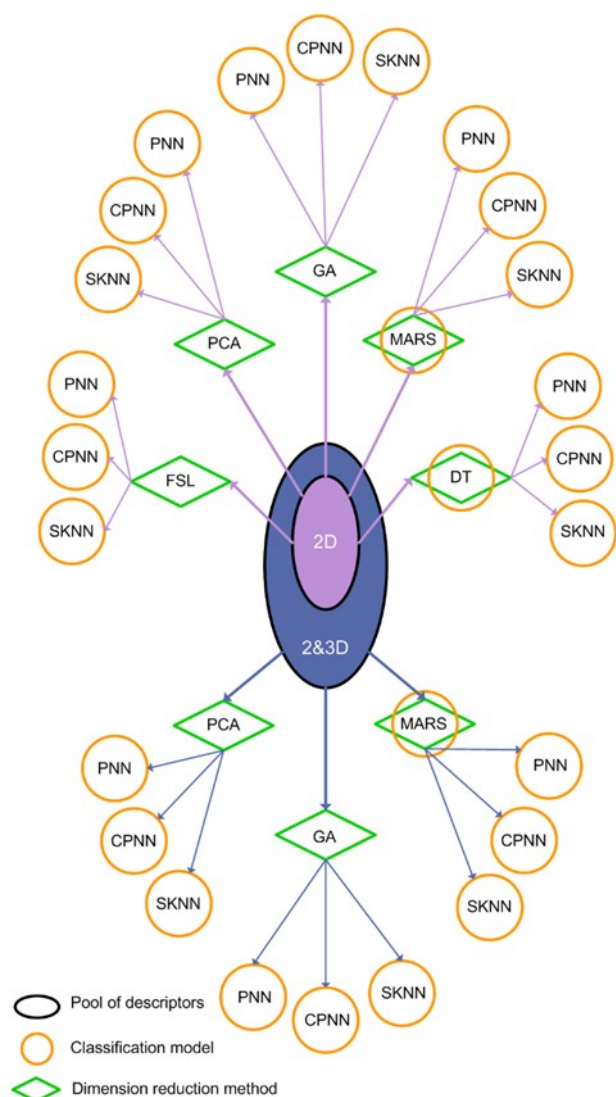
Figure 2. A schematic summary of the applied techniques and developed classification models
