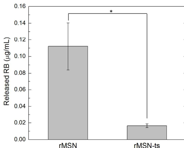
Fig. 6 Rose Bengal release from rMSN and rMSN-ts after incubating the particles (6 mg/mL) in PBS for 3 d. Error bars are standard deviation. *indicates p < 0.05 according to the student's t-test.
