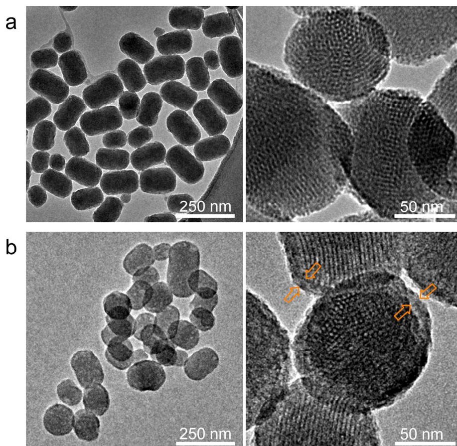
Fig. 2 TEM images of the surfactant containing MSNs; (a) rMSN and (b) rMSN-ts. Left and right panels show the low and high magnification images of the particles, respectively. Both particles have short rod-like shape and fairly monodisperse in size. Uniform silica layer around rMSN-ts can be easily observed from the images. Orange arrows in (b) indicate the nonporous shells formed around the mesoporous cores of rMSN-ts.
