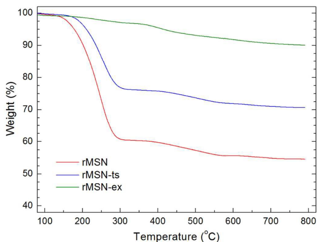
Fig. 3 TGA curves of the rMSN, rMSN-ts and rMSN-ex.
