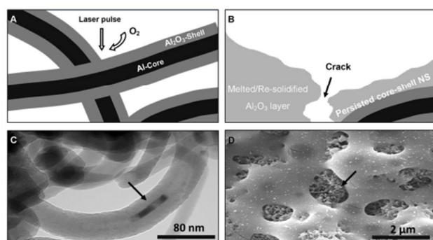
Fig. 2 (A) Schematic presentation of the laser assisted oxidation and transformation to \text{Al}_2\text{O}_3 , (B) Schematic presentation of the crack formation and melt flow/solidification \text{Al}_2\text{O}_3 layer, (C) TEM image of as-deposited 1D nanostructures with core-shell morphology (arrow shows core-shell structure) and (D) SEM image of deposited layer after the laser treatment (arrow shows the persisted nanostructures below the molten and re-solidified \text{Al}_2\text{O}_3 layer).
