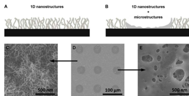
Fig. 1 Schematic presentation of (A) as deposited layer (nanostructured surface) and (B) laser treated layer (micro-/nanostructured surface). SEM images of (C) as deposited layer (nanostructured surface), (D) laser treated layer (micro-/nanostructured surface) and (E) inner surface of a micro-crater.
