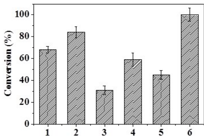
Fig. 6 Comparative lipase enzyme activity for the esterification of oleic acid with n-butanol (in terms of conversion of oleic acid). 1. Lipase dissolved in de-ionized water, 2. Lipase dissolved in butanol, 3. Self-assembled lipase in [Bmim][BF 4 ], 4. Self-assembled lipase capsules synthesized in [Bmim][PF 6 ], 5. Lipase encapsulated solid silica nanospheres synthesized in [Bmim][BF 4 ], 6. Lipase encapsulated in hollow silica nanocapsules synthesized in [Bmim][PF 6 ].
