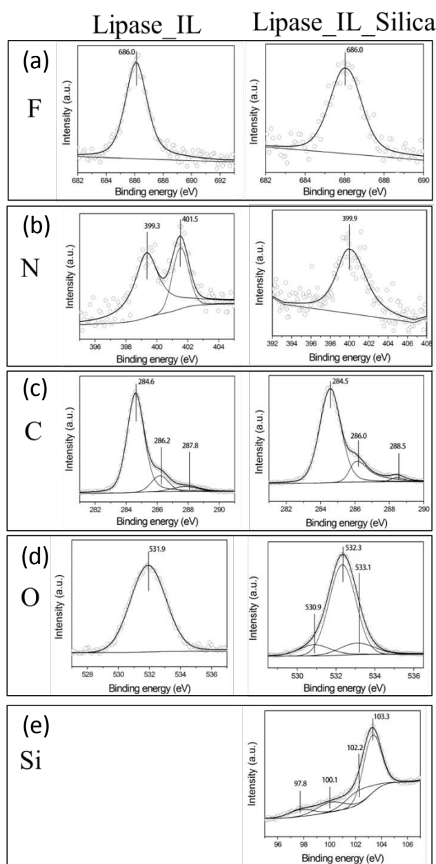
Fig. 3. XPS core-level spectra recorded from lipase and Lipase-Silica after interaction with ionic liquid [Bmim][PF 6 ]. (a) F 1s core-level spectra. (b) N 1s core-level spectra. (c) C 1s core-level spectra (d) O 1s core-level spectra (e) Si 2p from Lipase-IL and Lipase-IL-silica nanostructures. The solid lines correspond to nonlinear least-squares fits to the experimental data as shown by symbols.
