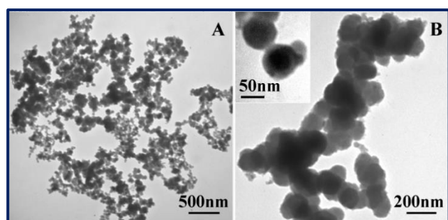
Fig. 5 Lower (A) and higher magnification (B) TEM images of solid silica nanoparticles synthesized in ionic liquid [Bmim][BF 4 ] using 20 \mu\text{g mL}^{-1} lipase enzyme.
