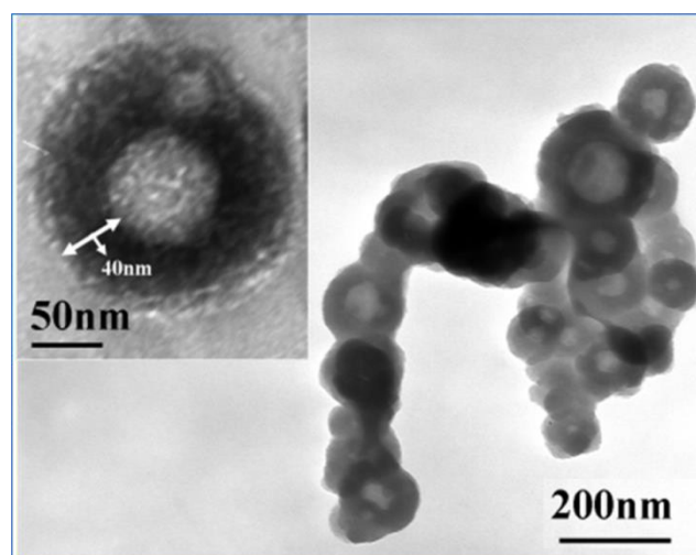
Fig. 2 TEM images of hollow silica nanoparticles synthesized in ionic liquid [BMIM][PF 6 ] using self-assembled lipase capsules as catalytic templates. Lipase template capsules were self-assembled using 20 \mu\text{g mL}^{-1} lipase enzyme and inset shows the thickness of hollow silica nanoparticles ( \sim 40 nm) at a higher magnification image of one of the particles from the same sample.
