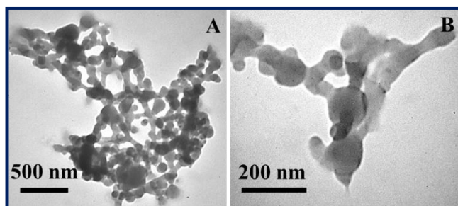
Fig. 4 Lower (A) and higher magnification (B) TEM images of self-assembled lipase ( 20 \mu\text{g mL}^{-1} ) structures obtained in ionic liquid [BMIM][BF 4 ].
