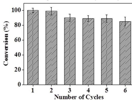
Fig. 7 Reusability study of lipase enzyme encapsulated within hollow silica nanospheres during their synthesis in ionic liquid [Bmim][PF 6 ] for esterification of oleic acid with 1-butanol.
