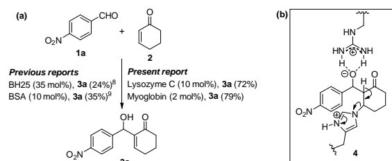
Figure 1. (a) Biocatalysis in MBH reaction. (b) Hypothetical activation of nucleophile and electrophile in a Michael addition - aldol condensation sequence (MBH) draws comparison with the catalytic activity of lipases. 11
