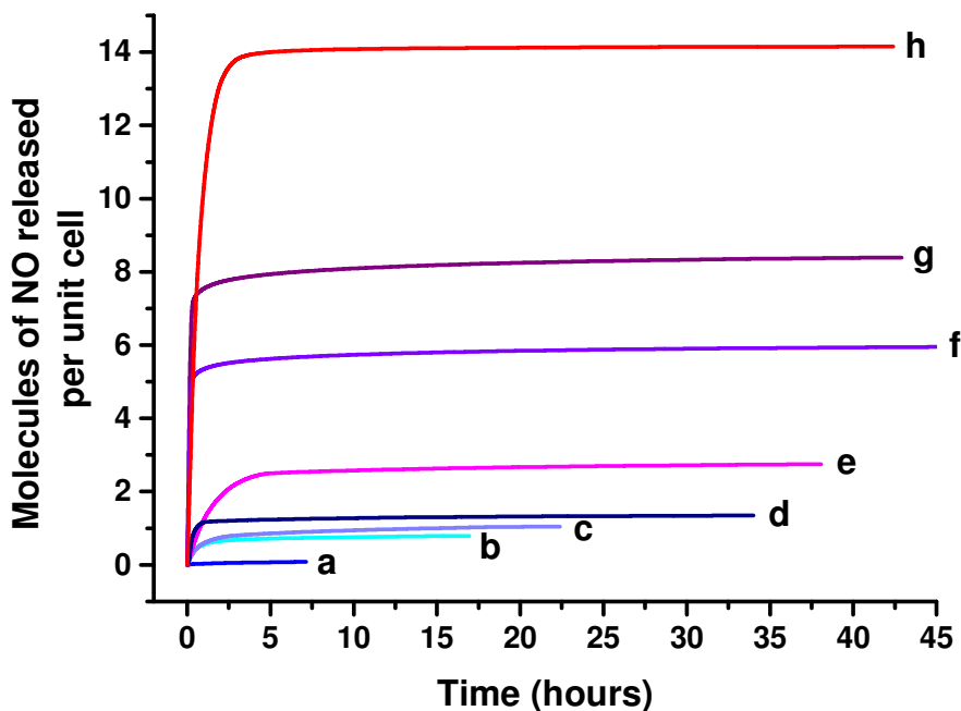
Figure 6: Chemiluminescence analysis of total NO delivery on contact with humid atmosphere (11% RH) for (a) CPO-27 (Mg), (b) CPO-27 (Mg) 1% Ni, (c) CPO-27 (Mg) 2% Ni, (d) CPO-27 (Mg) 5% Ni, (e) CPO-27 (Mg) 10% Ni, (f) CPO-27 (Mg) 20% Ni, (g) CPO-27 (Mg) 40% Ni and (h) CPO-27 (Ni). Data collection was stopped when NO levels reached 20ppb.
