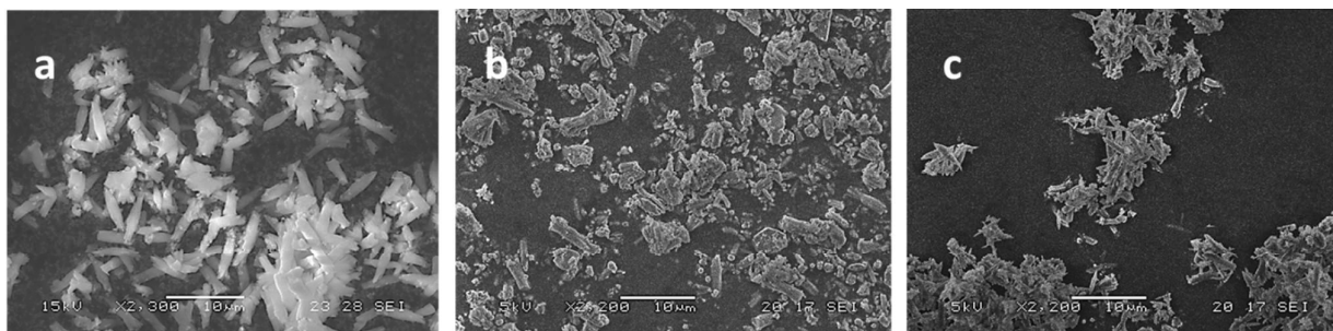
Figure 10: SEM images of (a) CPO-27 (Zn), (b) CPO-27 (Zn) 10% Ni and (c) CPO-27 (Zn) 20% Ni.
