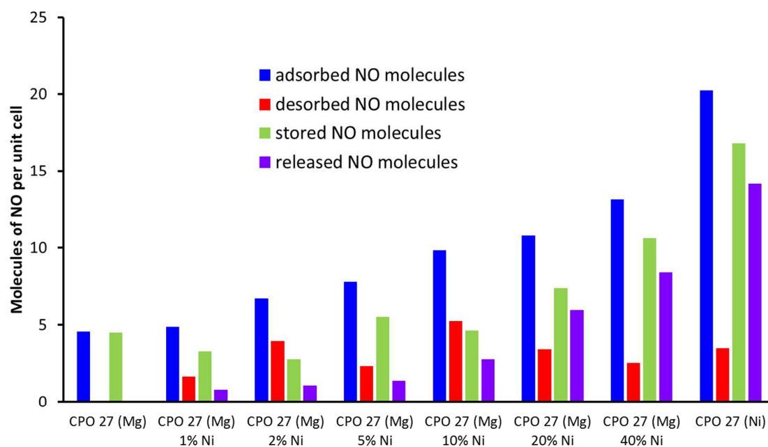
Figure 8: Total adsorbed (blue), desorbed (red), stored (green) (measured using a gravimetric adsorption system) and released Nitric Oxide (purple) at 298 K (measured using chemiluminescence analysis) for (a) CPO-27 (Mg), (b) CPO-27 (Mg) 1% Ni, (c) CPO-27 (Mg) 2% Ni, (d) CPO-27 (Mg) 5% Ni, (e) CPO-27 (Mg) 10% Ni, (f) CPO-27 (Mg) 20% Ni, (g) CPO-27 (Mg) 40% Ni and (h) CPO-27 (Ni).
