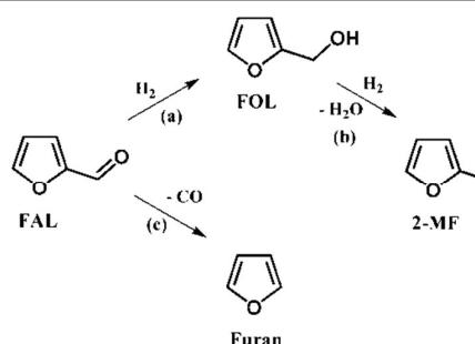
Scheme 1. Reaction routes for the hydrogenation of FAL to FOL and other possible products. (a) Hydrogenation, (b) hydrogenolysis, and (c) decarbonylation.
