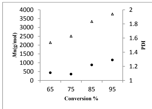
Figure 8. M_n ( \Delta ) and M_w/M_n ( \bullet ) vs. monomer conversion in the ROP of L -LA.
