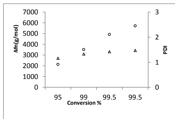
Figure 7. M_n (●) and M_w/M_n (▲) vs. monomer conversion in the ROP of \epsilon -CL.
