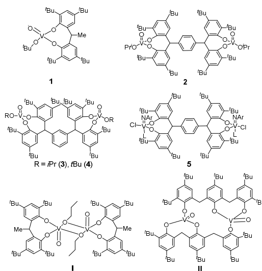
Scheme 1. Vanadyl complexes screened herein (Ar = p -tolyl, L = MeCN).
