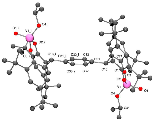
Figure 2. Molecular structure of 2 . Selected bond lengths (Å) and angles (°): V(1) – O(1) 1.575(4), V(1) – O(2) 1.777(4), V(1) – O(3) 1.750(5), V(1) – O(4) 1.759(5); O(2) – V(1) – O(3) 109.4(2), V(1) – O(2) – C(1) 139.7(5), V(1) – O(3) – C(17) 151.7(4), V(1) – O(4) – C(40) 130.1(5).
