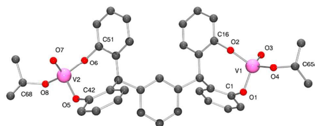
Figure 3. Molecular structure of complex 3 ·2CH 2 Cl 2 , indicating the atom numbering scheme. Hydrogen atoms have been removed for clarity.
