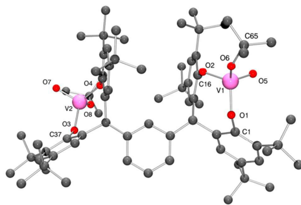
Figure 4. Molecular structure of complex 4 ·2CH 2 Cl 2 , indicating the atom numbering scheme. Hydrogen atoms have been removed for clarity.
