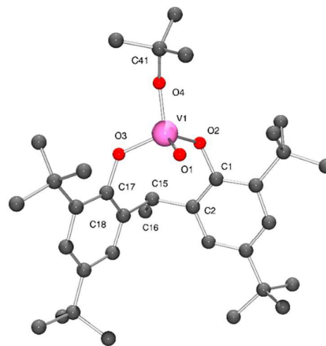
Figure 1. Molecular structure of 1 . Selected bond lengths ( \text{\AA} ) and angles ( ^\circ ): V(1) - O(1) 1.789(5), V(1) - O(2) 1.783(5), V(1) - O(3) 1.581(5), V(1) - O(4) 1.739(5); O(1) - V(1) - O(2) 110.1(2) , V(1) - O(1) - C(1) 124.4(4) , V(1) - O(2) - C(17) 130.9(4) , V(1) - O(4) - C(41) 145.9(5) .
