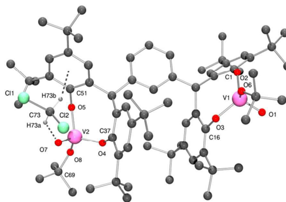
Figure 5. Molecular structure of complex 4·3CH 2 Cl 2 , indicating the atom numbering scheme. Hydrogen atoms have been removed for clarity.
