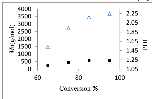
Fig 9. M_n (Δ) and M_w/M_n (●) vs. monomer conversion in the ROP of rac -LA.
