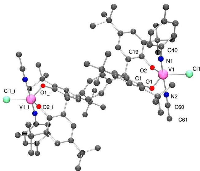
Figure 6. Molecular structure of complex 5 ·2MeCN, indicating the atom numbering scheme. Hydrogen atoms have been removed for clarity. Selected bond lengths (Å) and angles (°): V(1)–N(1) 1.670(3), V1–O1 1.818(3), V1–O2 1.831(2), V1–Cl1 2.2609(11); O1–V1–N1 98.33(13), O1–V1–O2 111.59(11), Cl1–V1–N1 94.74(11), V1–O1–C1 124.4(2), V1–O2–C19 121.4(2), V1–N1–C50 170.5(3). Symmetry operation used to generate equivalent atoms: i = – x , – y , – z .
