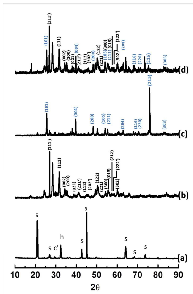
Figure 6. XRD patterns of (a) concrete, where s, c' are h are corresponding reflections for SiO 2 , CaCO 3 and Ca(OH) 2 respectively (b) ZrO 2 NP doped concrete, (c) TiO 2 NP doped concrete, (d) concrete with both TiO 2 & ZrO 2 NPs. Broad peaks observed for TiO 2 and ZrO 2 are indicative of nanoparticles
