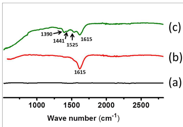
Figure 8. Infrared Spectra of (a) concrete, (b) concrete with PAA, (c) concrete-PAA-U, in C, spectral bands at 1525, 1441 and 1390 \text{cm}^{-1} are due to N-H deformation, in plane O-H bending and C-H bending modes, along with lowering in intensity of COO- asymmetric stretching mode in PAA is indicative of supramolecular interaction between PAA and urea
