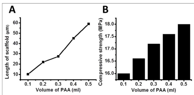
Figure 4. (A) Quantification of scaffold length with variation of PAA volume at fixed U amount, (B) Comparison of compressive strength of concrete systems with variation of PAA volume
