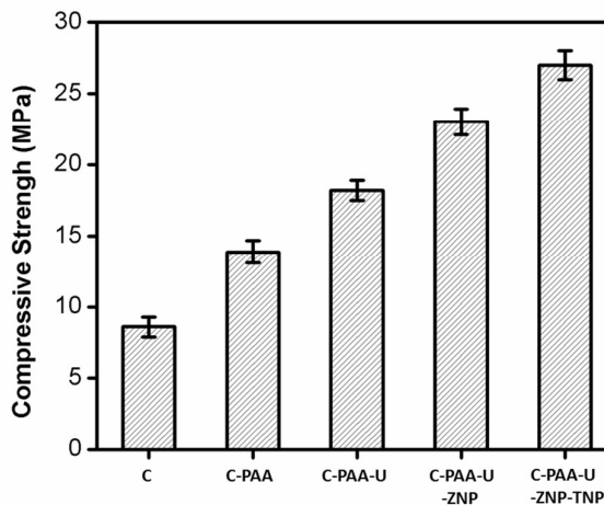
Figure 2. Comparison of compressive strength of the samples, significant enhancement of compressive strength is observed with inclusion of scaffolds. Further enhancement is seen with incorporation of ZrO_2 & TiO_2 NPs
