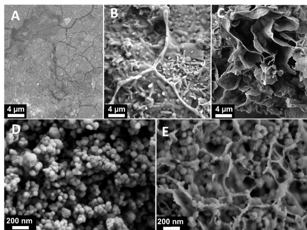
Figure 1. SEM images of (A) concrete matrix, (B) struts formed by PAA in concrete matrix, (C) PAA-Urea supramolecular scaffolds, (D) ZrO_2 and TiO_2 nanoparticles in concrete with no scaffolds and (E) ZrO_2 and TiO_2 nanoparticles within scaffolds, size of ZrO_2 and TiO_2 nanoparticles has been determined to be 54 and 30 nm, respectively, by using a scale bar inside SEM
