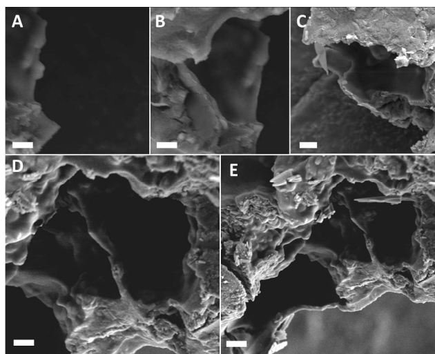
Figure 3. (A-E) Increased scaffold length with increase in concentration of PAA for a fixed U concentrations, scale bar represents 2 \mu\text{m} in all images
