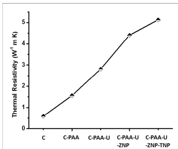
Figure 7. Comparison of thermal resistivity of the samples, thermal resistivity increases with inclusion of defects/dislocations.
