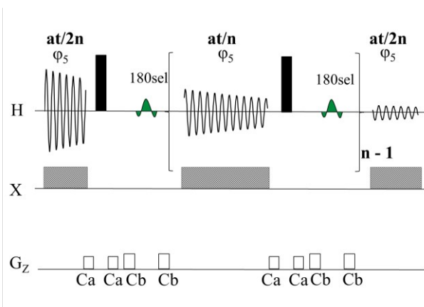
Figure 3: Band-selective J -refocussing element incorporated into the t_2 acquisition period for band-selective homodecoupling. The 180sel pulse (green) is a refocussing 180^\circ RSNOB.
