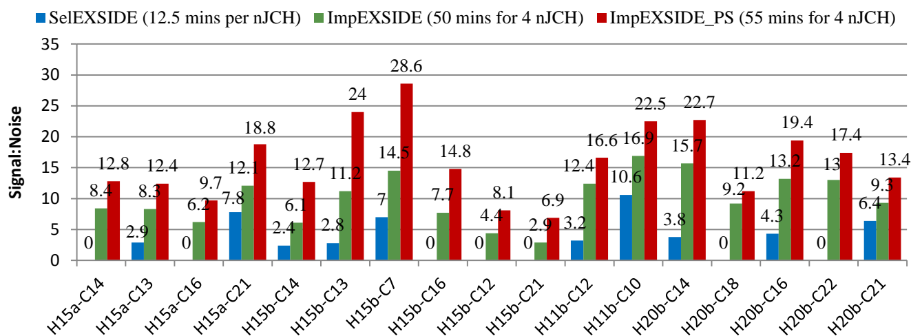
Figure 2: The signal to noise ratio of peaks arising from heteronuclear coupling of H15a/b, H11b and H20b of strychnine from SelEXSIDE (blue), ImpEXSIDE (green) and Pure-shift ImpEXSIDE (red).
