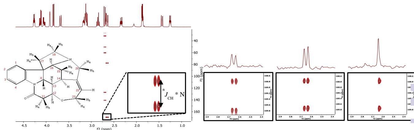
Figure 1: Strychnine structure and H11b-C10 correlations from the corresponding (a) H20b/H11b EXSIDE spectrum (~ 7.5 hours) with H11b – C10 inset. (b) SelEXSIDE spectrum (50 minutes) (c) ImpEXSIDE spectrum (50 minutes, as one of four correlations measured simultaneously) and (d) ImpEXSIDE_PS spectrum (50 minutes, as one of four correlations measured simultaneously).
