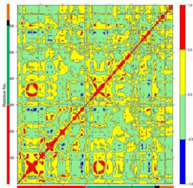
Figure 5 The Dynamic Cross Correlation Analysis (DCCA) of wild type TPST-2. Protomer A and B, substrate peptide and cofactor are represented in red, green, black and orange colours respectively. The positive correlated motion is shown in red colour and the negative correlated motion in blue colour. The analysis was done using R Bio3D package 35 .
