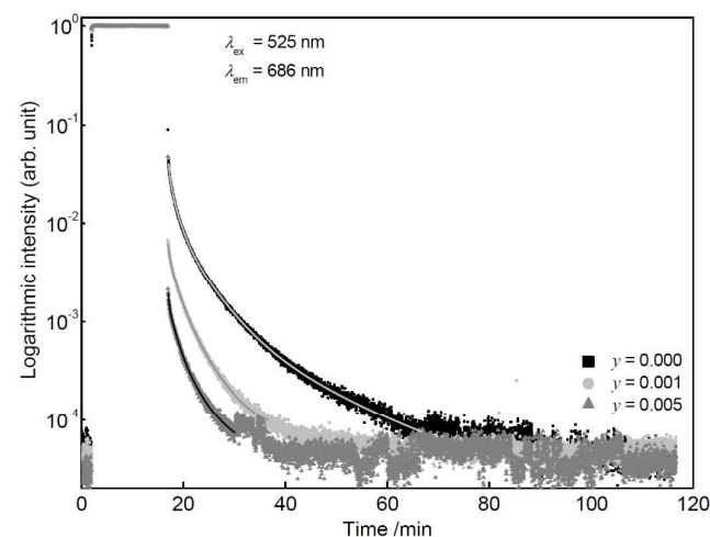
Fig. 10 PLD curves of \text{Sr}_{0.999-y}\text{Eu}_{0.001}\text{Dy}_y\text{Sc}_2\text{O}_4 with different concentrations of \text{Dy}^{3+} .
