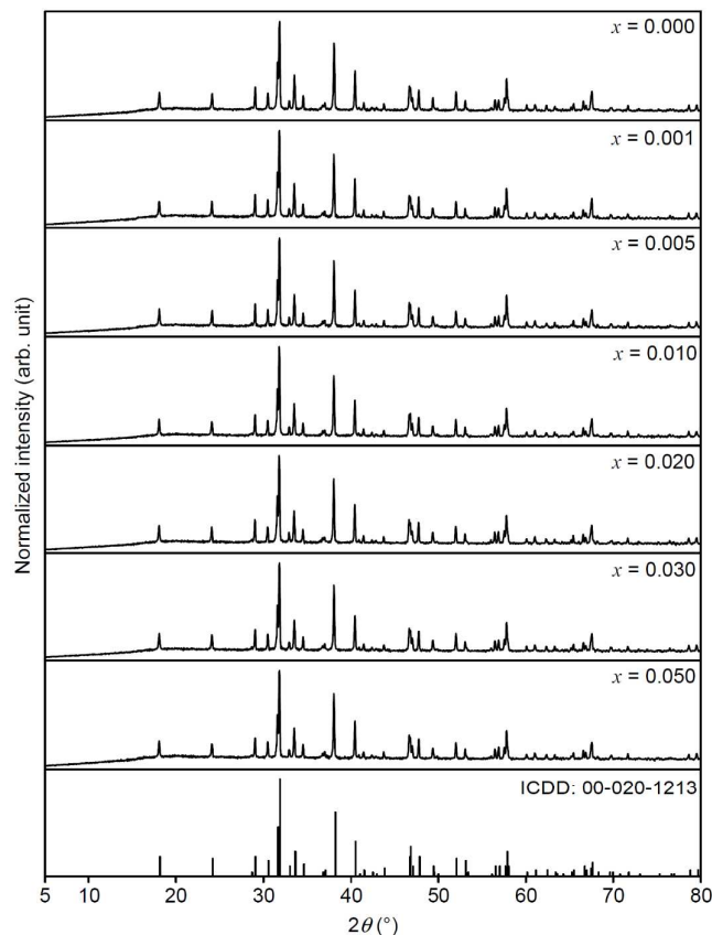
Fig. 1 XRD patterns of \text{Sr}_{1-x}\text{Eu}_x\text{Sc}_2\text{O}_4 with various doping concentrations and ICDD reference card of \text{SrSc}_2\text{O}_4 .
