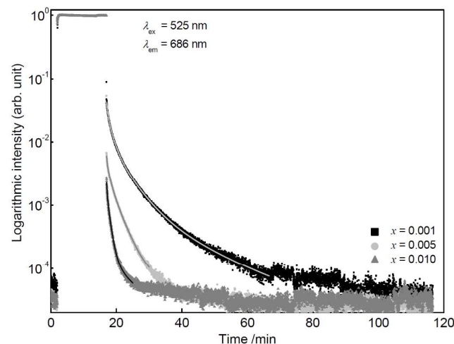
Fig. 9 PLD curves of \text{Sr}_{1-x}\text{Eu}_x\text{Sc}_2\text{O}_4 with various doping concentrations.
