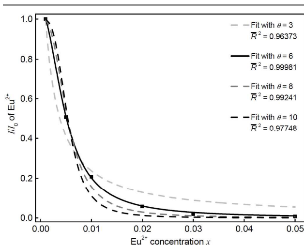
Fig. 7 Dependence of I/I_0 on the \text{Eu}^{2+} concentration.
