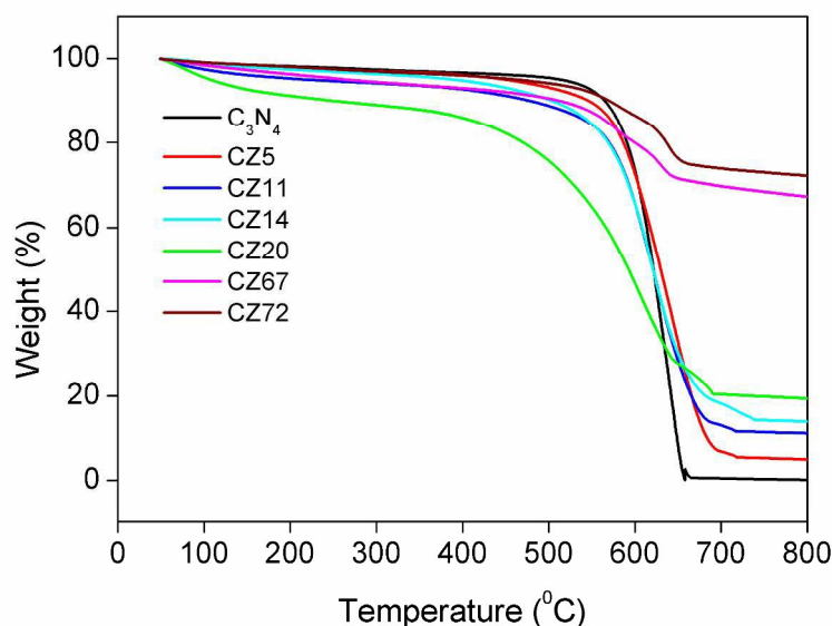
Fig. 1 Post synthesis TGA of C_3N_4 -ZnS compositions
