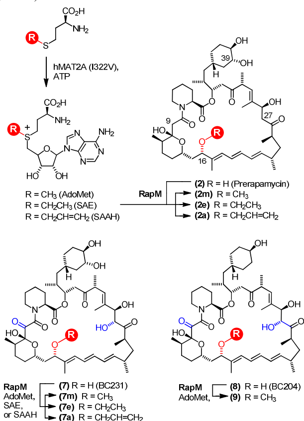
Fig. 2. Enzymatic production of AdoMet analogues by MAT and alkylation of rapalogs by RapM. The hMAT2A mutant I322V utilises ATP and methionine analogues to produce AdoMet analogues carrying methyl (AdoMet), ethyl (SAE) and allyl (SAAH) substituents on the sulphonium centre. The AdoMet analogues are subsequently used by RapM to transfer alkyl groups to the rapalog substrates prerapamycin (BC150) 2 and BC231 7 , generating methyl ( m ), ethyl ( e ) and allyl ( a ) derivatives.
