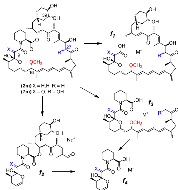
Fig. 4. MS n fragmentation pattern for rapalogs, showing the defined product ions f 1 , f 2 , f 3 and f 4 . The RapM site of methylation can be identified by comparing the f 1 and f 2 ions for rapalogs 7 , 7m and 2 , 2m .
