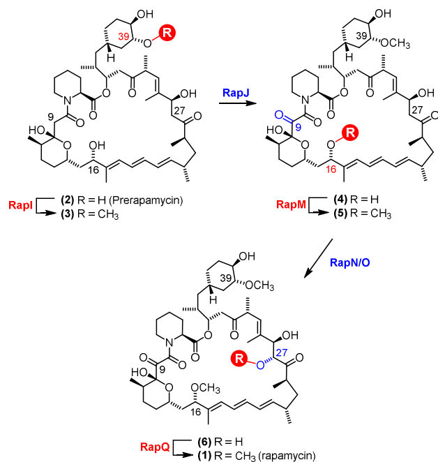
Fig. 1. Proposed modification of prerapamycin 2 by tailoring enzymes. 18 The first post-PKS intermediate 2 is assembled by three PKSs RapA, B and C and cyclised by the pipecolate-incorporating NRPS-like enzyme RapP. Subsequent modification of the macrocycle occurs by methylation at the 16, 27 and 39- O -positions by three O -methyltransferases RapM, RapQ and RapI. Two P450 monooxygenases RapJ and RapN serve to introduce a keto-group and hydroxyl-group at the C9 and C27 positions respectively. RapQ methylates only after hydroxylation at C27 by RapN.
