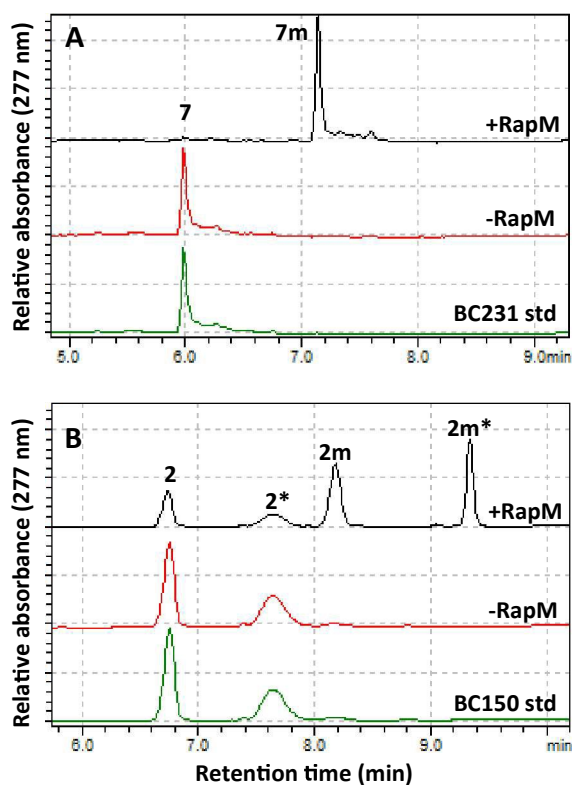
Fig. 3. HPLC analyses of BC231 ( 7 ) and BC150 ( 2 ) assays with AdoMet. A: RapM assay with BC231 7 , showing formation of the methyl product 7m . B: RapM assay with BC150 2 and 2* (rotamers), showing formation of dual peaks corresponding to rotamers of the methylated product ( 2m , 2m* ).
