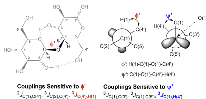
Scheme 2. Torsion angles ( \phi' and \psi' ) across the 1,4- \beta -glycosidic bond and the respective J-couplings sensitive to \phi' and \psi' according to Ref. 48 . The current representation of cellobiose does not correspond to an optimised structure. Dashed lines indicate the O(5) \cdots HO(3') and O(2)H \cdots O(6') intramolecular H-bonds.
