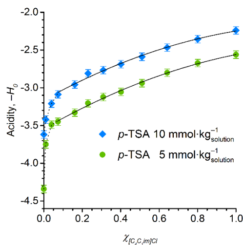
Fig. 5. Acid strength of p -TSA in DMSO, [C 4 C 1 im]Cl/DMSO mixtures, and [C 4 C 1 im]Cl at 25 °C. In all the media, a 2 wt% concentration of water is present to correspond to the reaction media of cellulose depolymerisation and cellobiose hydrolysis. The self-acidity of [C 4 C 1 im]Cl/DMSO mixtures corresponds to H 0 values of 4.4 ± 0.1.
