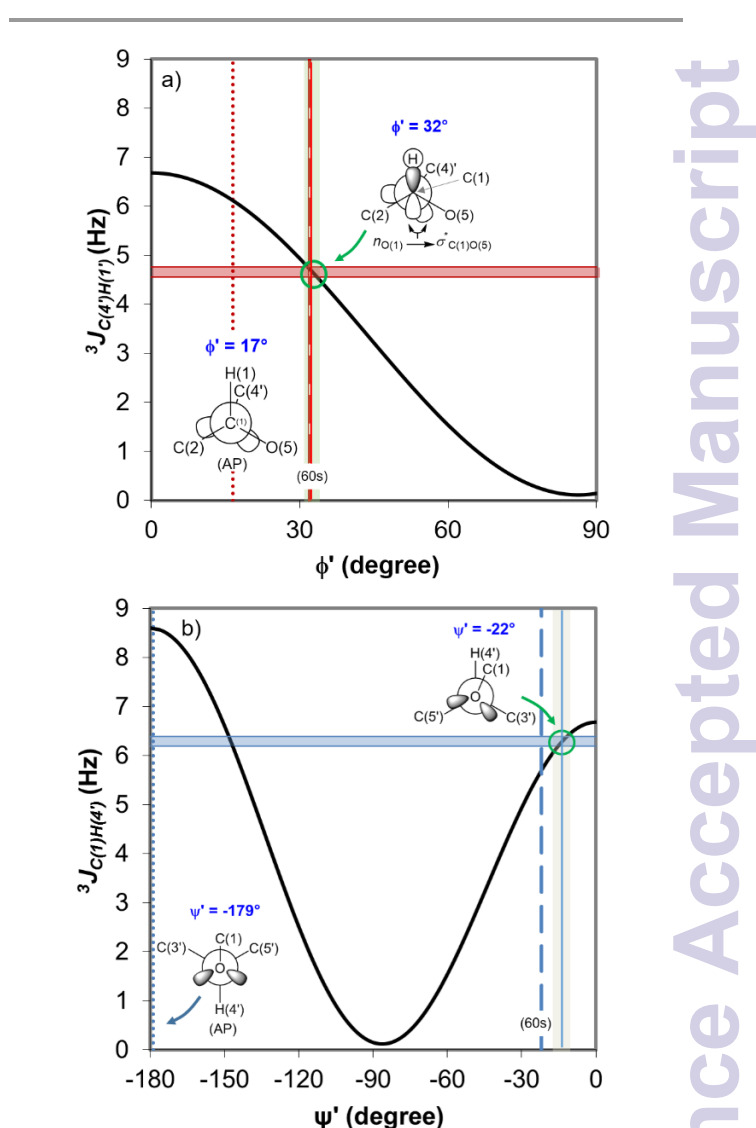
Fig. 4 DFT-predicted Karplus curve (black) for 3-bond scalar ( {}^3J_{CH} ) coupling as a function of torsion angle -C-O-C-H- according to Cloran et al. 48 Red and blue solid horizontal lines correspond to the average coupling constants, {}^3J_{C(4'),H(1)} (Fig. 4a) and {}^3J_{C(1),H(4')} (Fig. 4b) measured for cellobiose in DMSO- d_6 and [C_4C_{1im}]Cl-d_{15}/DMSO-d_6 binary solutions at 90 °C. Lowest energy torsion angles for the so-called "60s" (dashed, [\varphi, \psi] = [32^\circ, -22^\circ] ) and for the "AP" conformations (dotted, [\varphi, \psi] = [17^\circ, -179^\circ] ) also represented, 50 The measured couplings intercept the Karplus curve very close to the areas corresponding to the "60s" conformation, based on DFT calculations (green circle). 48
