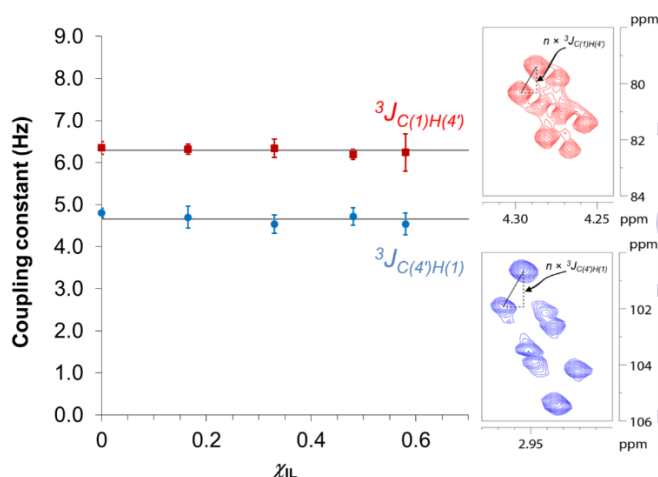
Fig. 3. Dependence of HR-HMBC3 heteronuclear long-range coupling across the glycosidic bond with ionic liquid molar fraction. Inset: Cross-peaks in the HR-HMBC3 spectrum from which the coupling was measured. The vertical displacement of peak pattern corresponds to the coupling constant value multiplied by a scaling factor (here, n=25 ). Hence, J_{CH} values were obtained from the value of vertical displacement divided by 25. Solid grey lines represent the ^3J_{CH} coupling averaged values considering the coupling constants in the indicated solvent compositions ( 4.7 \pm 0.1 Hz and 6.3 \pm 0.1 Hz).
