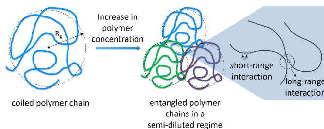
Scheme 1. Representation of a coiled polymer chain, which is characterised by a hydrodynamic gyration radius ( R_g ), and the entangled state of neighbouring polymer chains in a semi-diluted regime. For clarity, different colours were used in order to represent the different chains of the same polymer in the entangled state.
