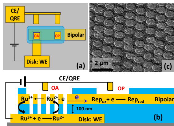
Figure 1. (a) Schematic diagram showing a top view of the macroscopic layout of the BRDE array and remote electrode separated by mm-distances; (b) Schematic side view of the BRDE array and illustration of the mechanism of self-induced redox cycling for Ru(NH_3)_6^{2/3+} (abbreviated as Ru^{2/3+} ). SIRC in the BRDE at OA is monitored by a reporter redox couple ( Rep_{ox/red} ) at a remote location (OP); (c) SEM image of the array at 45° tilt.
