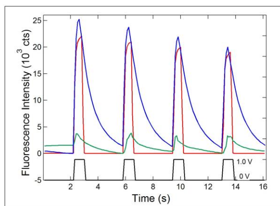
Figure 4. Comparison of electrochemically-induced fluorescence and SIRC-coupled fluorescence in solutions of 0.1 mM dihydroresorufin at the OP portion of the bipolar electrode. Potential steps between 0 V and 1.0 V vs. QRE (black) were applied at the recessed disk electrode array (OA) filled with 100 \mu\text{M} (blue) and 1 \mu\text{M} (green) ferrocenemethanol solutions in a PDMS well. Red curve: Potential steps applied directly to the bipolar electrode at OP with no solution in the OA portion of the bipolar electrode. (Intensity x 0.1).
