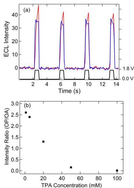
Figure 3. (a) ECL measurement in 5 mM \text{Ru}(\text{bpy})_3^{2+} and 5 mM TPA solutions on the multiscale bipolar electrode at OA (blue) and OP (red) in the same PDMS well. Multiple potential steps switching between 1.8 V and 0 V vs. QRE (black) were applied on the disk with the bipolar electrode floating. (b) Ratio of ECL intensities at OP and OA as a function of TPA concentration.
