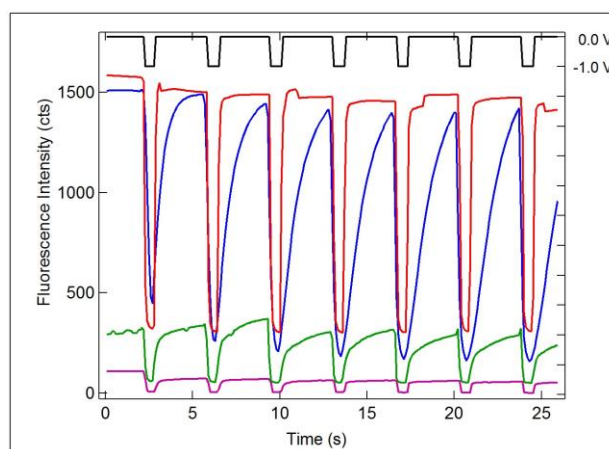
Figure 5. Comparison of electrochemically-induced fluorescence and SIRC-coupled fluorescence in solutions of 0.1 mM resorfin at the OP portion of the bipolar electrode. Potential steps between 0 V and -1.0 V vs. QRE (black) applied at the recessed disk WE at OA for 1 mM (blue), 1 μM (green), and 1 nM (purple) Ru(NH 3 ) 6 3+ in a PDMS well. Red curve: Potential steps applied directly to the bipolar electrode at OP with no solution covering the OA portion of the bipolar electrode (Intensity displayed at 0.03x). Offsets used to enhance visualization.
