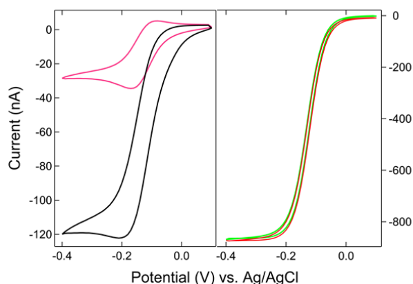
Figure 2. (Left) Cyclic voltammograms of 1 mM \text{Ru}(\text{NH}_3)_6^{3+} on a BRDE array with only OA contacting solution (black) and on a recessed microdisk electrode array of the same size (pink). (Right) CVs on the array with both OA and OP (1 mm x 5 mm) in contact with 1 mM \text{Ru}(\text{NH}_3)_6^{3+} . The bipolar electrode is floating (red) or held at +0.1 V (green), respectively, vs. Ag/AgCl.
