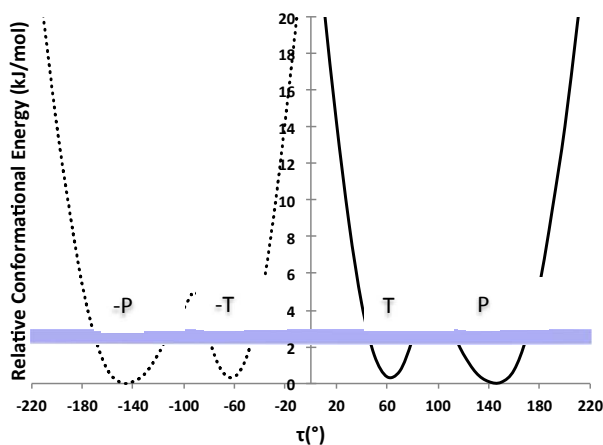
Figure 2. PES scan of TA tautomer A as a function of \tau in ethanol ( \tau step = 10°). Two curves are plotted (one per enantiomer) and RT at the crystallisation conditions is given as a blue band.
