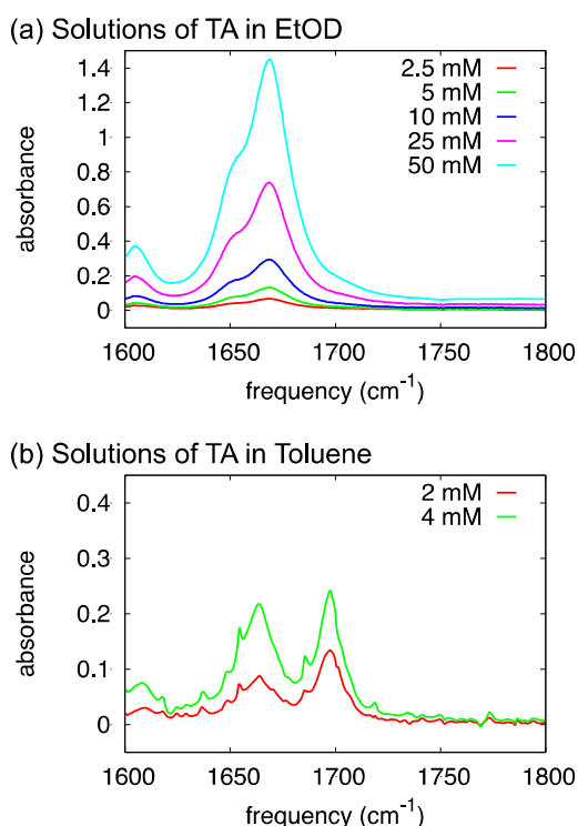
Figure 5. FTIR spectra of solutions of TA in deuterated ethanol (a) and toluene (b) at varying concentrations.
