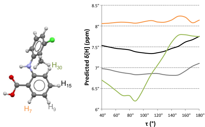
Figure 4. Calculated changes in chemical shifts with torsion angle \tau for four selected hydrogen atoms. H30 is the aromatic hydrogen atom displaying the most significant changes in chemical shift with molecular conformation.
