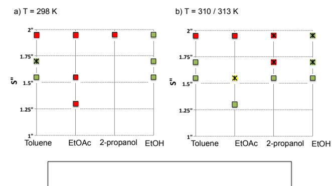
Figure 6. Crystallisation outcomes as a function of supersaturation and solvent at 298 and 310/313 K. Pure green and red squares correspond to experiments for which at least four out of the five crystallizations performed resulted in pure forms I and II respectively. Crossed squares represent mixed outcomes with a majority (at least three out of five crystallisations) of form I (green), II (red) or both (yellow, concomitant).
