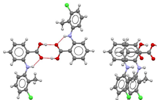
Figure 3. Hydrogen-bonded (left) and stacked (right) dimers of TA.
