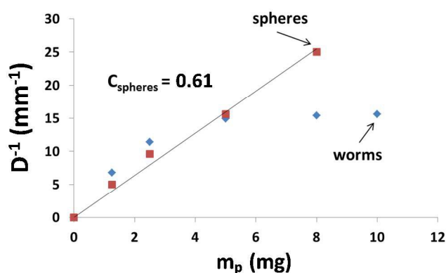
Figure 3. Effect of varying the copolymer particle mass m_p on the droplet diameter for two series of water-in- n -dodecane emulsions stabilised using (a) PLMA 16 -PBzMA 37 spheres (red squares) and (b) PLMA 16 -PBzMA 37 worms (blue diamonds). Note the deviation from linearity for the latter particles.
