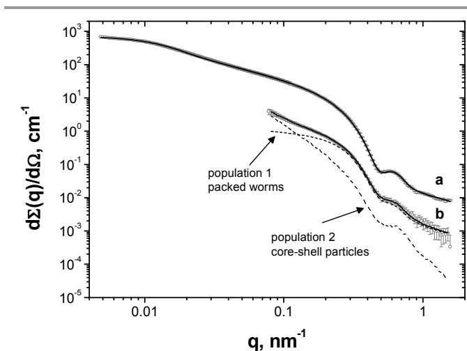
Figure 4. Experimental SAXS data (circles) and fitting curves (solid lines) of (a) a dilute (1.0 % w/w) PLMA 16 -PBzMA 37 worm dispersion in n -dodecane and (b) an emulsion comprising aqueous droplets in n -dodecane stabilised by PLMA 16 -PBzMA 37 worms. Two dashed curves indicate the relative contributions of each population to model 2 (adsorbed worms and core-shell particles) to the total scattering of the curve fit.
