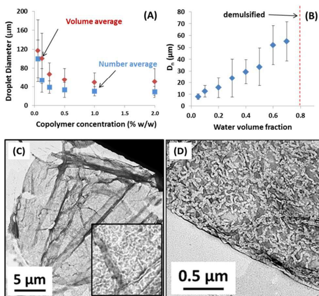
Figure 2. A) Water droplet diameter as a function of PLMA 16 -PBzMA 37 worm concentration in n -dodecane as determined by optical microscopy (number-average) and laser diffraction (volume-average). (B) Number-average water droplet diameter vs. water volume fraction for a fixed copolymer concentration of 0.50% w/w. (C, D) TEM images of the surface of a dried, collapsed Pickering emulsion droplet (using a 0.50% w/w worm concentration and a water volume fraction of 0.50) after evaporation of both the aqueous droplet phase and the n -dodecane continuous phase. The PLMA 16 -PBzMA 37 worms are clearly visible intact at the surface of this dried droplet.
