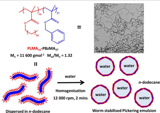
Figure 1. Preparation of Pickering emulsions prepared by homogenisation of PLMA 16 -PBzMA 37 diblock copolymer worm-like micelles dispersed in n -dodecane with an equal volume of water at 12 000 rpm for 2 minutes at 20 °C.
