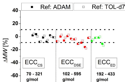
Fig. 5 ECC-MW-determination of a view model compounds at a concentration of 120 mM at 25°C. ADAM was used in equimolar concentration as internal reference.
