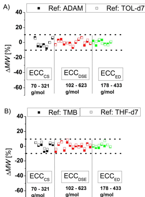
Fig. 3 Using A) ADAM/TOL- d_7 or B) TMB/THF- d_7 as internal reference (15 mM) gives a good MW-determination with a standard deviation of \sigma = 4\% . All of these model compounds were used to derive the ECCs.
