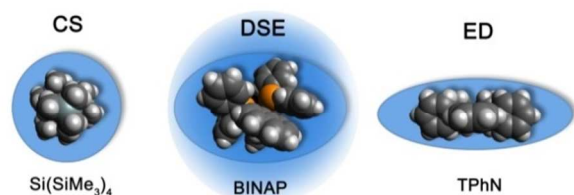
Fig. 2 Example molecules that were classified in our calibration curves as CS, DSE and ED like molecules
