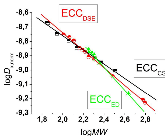
Fig. 1 \log D versus \log MW in TOL- d_8 . All compounds were normalized to \log D_{ref,fix} (ADAM) = -8.8454, see Table 4.
