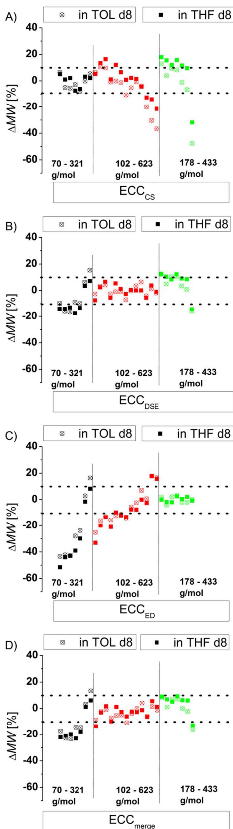
Fig. 4 Using exclusively A) ECC_{CS}^S , B) ECC_{DSE}^S , C) ECC_{ED}^S and D) ECC_{merge} on all model compounds (15 mM).
