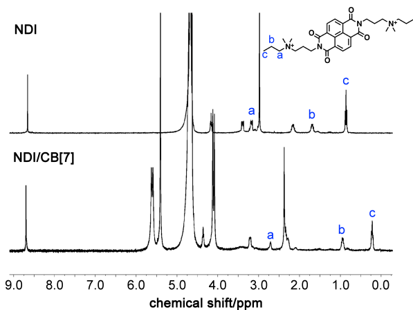
Figure 1. ^1\text{H} NMR spectra of NDI and NDI/CB[7] supramolecular complex (400 MHz, \text{D}_2\text{O} , 25^\circ\text{C} ).
