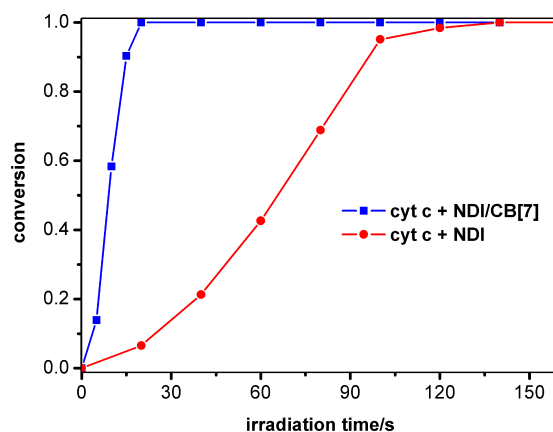
Figure 6. Reduction kinetics of cyt c at the existence of NDI or NDI/CB[7] supramolecular complex.
