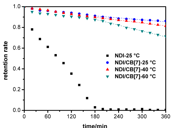
Figure 5. Stability of NDI and NDI/CB[7] monitored by UV/vis spectra.
