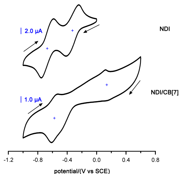
Figure 3. Cyclic voltammograms of NDI and NDI/CB[7].
