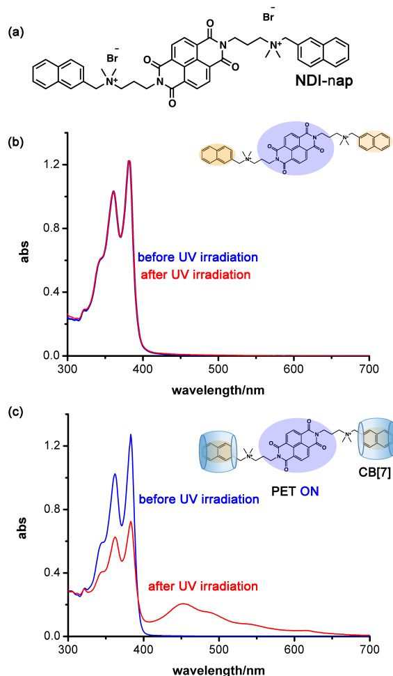
Figure 7. (a) Molecular structure of NDI-nap. (b) UV/vis spectra of NDI-nap before and after UV irradiation. (c) UV/vis spectra of NDI-nap/CB[7] before and after UV irradiation.
