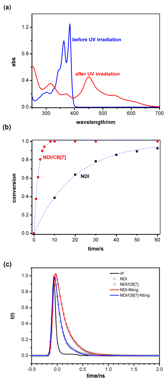
Figure 2. (a) UV/vis spectra of NDI/CB[7] before and after UV irradiation. (b) Reaction dynamics of NDI and NDI/CB[7] under UV irradiation. (c) Time-resolved fluorescence measurements of NDI and NDI/CB[7].
