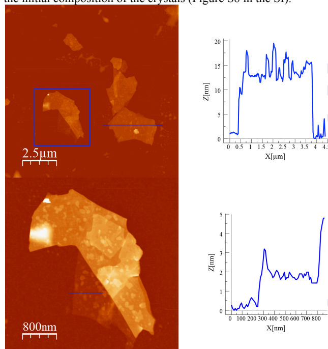
Figure 6. AFM images and height profiles of flakes of 2 shown in figure 5 obtained by mechanical exfoliation on a 285 nm \text{SiO}_2/\text{Si} substrate.
