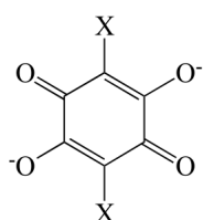
X 2 An 2- ; X = Cl or Br
