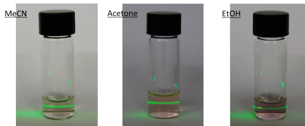
Figure 9. Tyndall effect of crystals of 2 after immersing in acetone, ethanol or acetonitrile (1.0 mg in 1 mL) overnight and then ultrasonicing for 1 minute.
