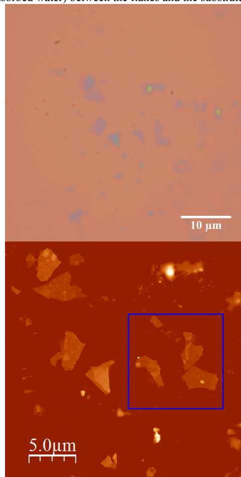
Figure 5. (a) Optical microscopy image (top) and AFM image of flakes of 2 obtained by mechanical exfoliation on a 285 nm \text{SiO}_2/\text{Si} substrate taken in the same zone (bottom).
