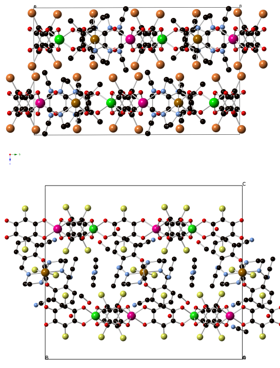
Figure 2. Projection of 2 (top) and 4 (bottom) in the bc plane (Fe (brown), Cr (green), Mn (pink) C (black), N (blue), O (red), Br (orange), Cl (yellow)). Hydrogen atoms have been omitted for clarity.
