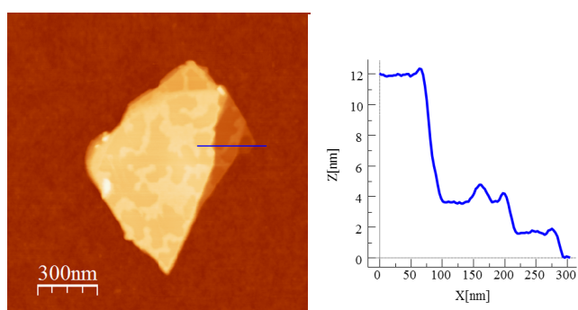
Figure 8. AFM image and height profile of a flake of 4 obtained by mechanical exfoliation on a 285 nm SiO 2 /Si substrate. Three nanosheets of about 2, 4 and 12 nm are discernible.
