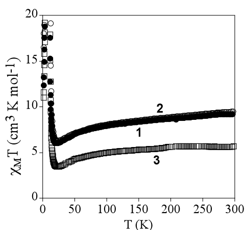
Figure 3. Temperature dependence of the product of the molar magnetic susceptibility times the temperature ( \chi_m T ) of 1 (full circles), 2 (empty circles) and 3 (empty squares) with an applied field of 0.1 mT.
