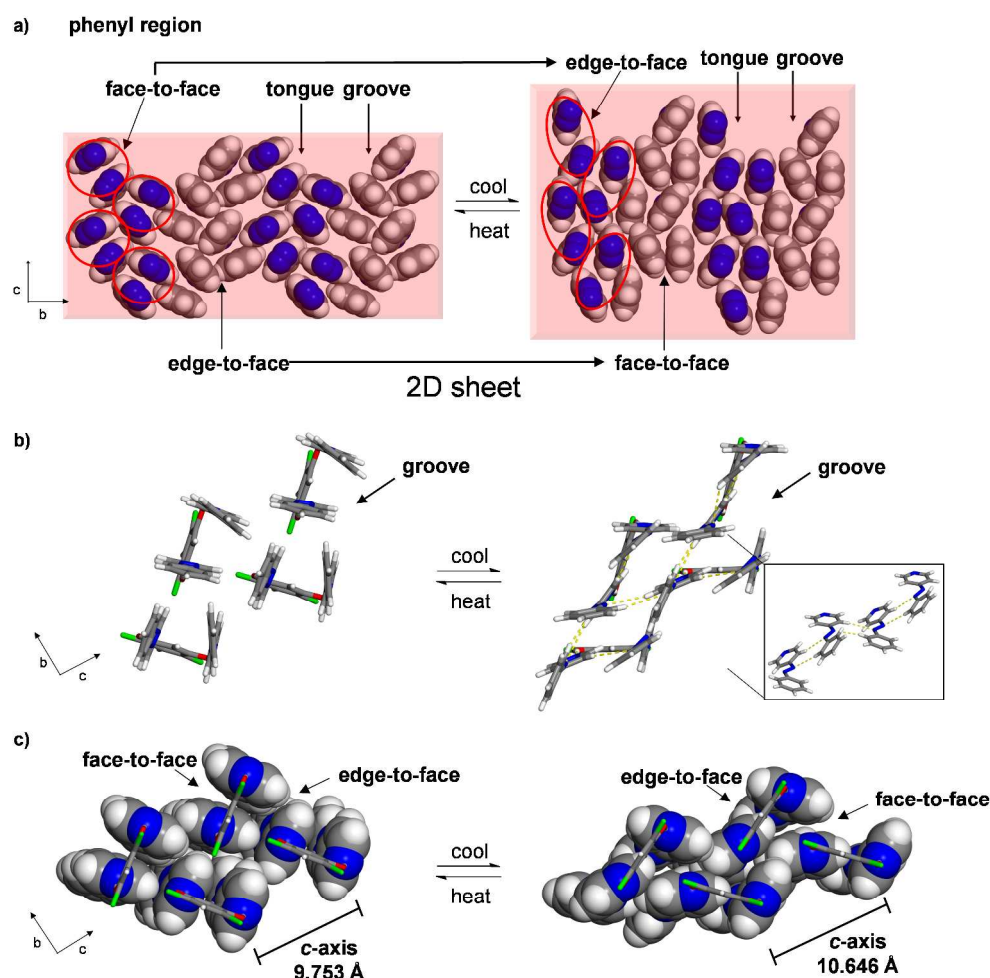
Fig. 5. Interconversion of \pi - \pi stacking in 1 (290 to 250 K): (a) 2D sheet (rotation of phenyl region by 60° relative to Scheme 1; circles highlight azo groups of an assembly), (b) C-H \cdots N interactions (yellow dotted lines, inset shows step-like structure) and (c) interconversions between edge-to-face and face-to-face \pi - \pi packings within a groove (resorcinol axle shown in wireframe).
