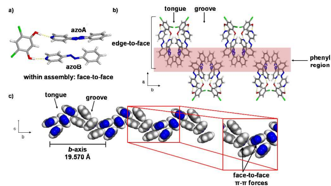
Fig. 3 Co-crystal 1 at 290 K: (a) three-component assembly, (b) edge-to-face forces that define tongue-and-groove, and (c) end-on view of face-to-face forces within assemblies (blue = azo group).
