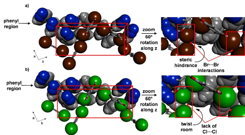
Fig. 7 Crystal structures at 290 K highlighting role of halogen interactions in phenyl region of: (a) 2 and (b) 1 (right provides insets).
