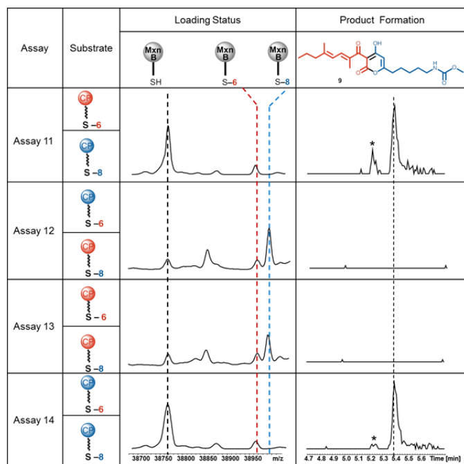
Fig. 6 LC-MS analysis of competition assays at 1 min. Competition Assay 11 (MxnB, 6-CP-W, 8-CP-E), Assay 12 (MxnB, 8-CP-W and 6-CP-E), Assay 13 (MxnB, 6-CP-W, 8-CP-W) and Assay 14 (MxnB, 6-CP-E and 8-CP-E). Competition assays were performed in a time course of 15 s to 10 min observing transfer of substrate to MxnB (loading status). EIC of 9 at [M+H]^+ = 406.22 for product formation are shown. Peak with asterisk (*) is the isomer of 9.
