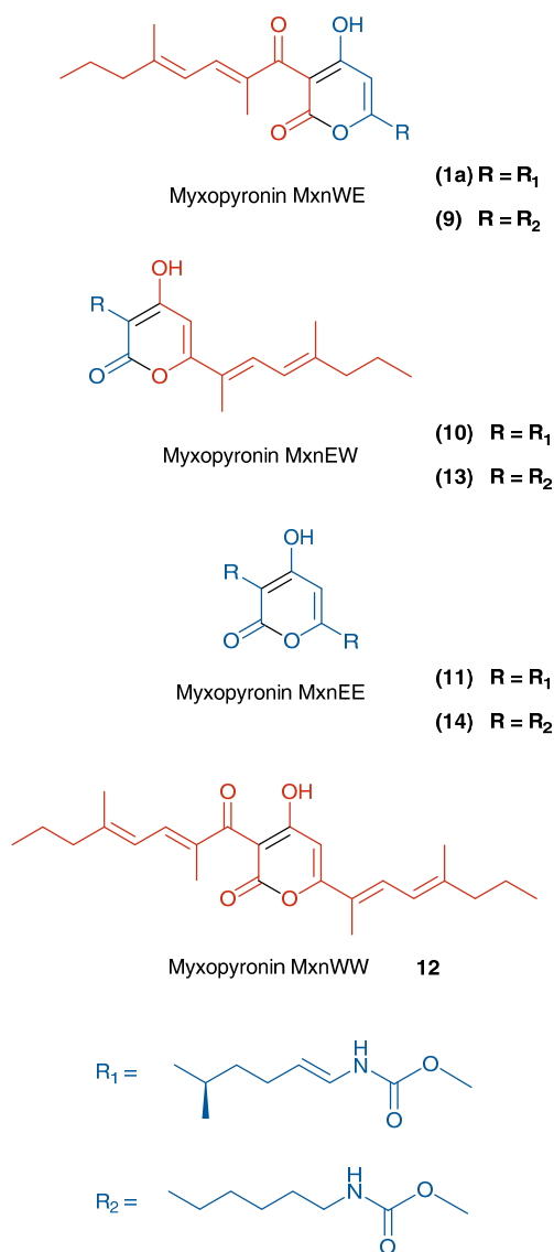
Fig. 5 Compounds produced by the myxopyronin wild type producer and in the scope of in vitro assays. Red represents the western chain, blue represents the eastern chain and black
