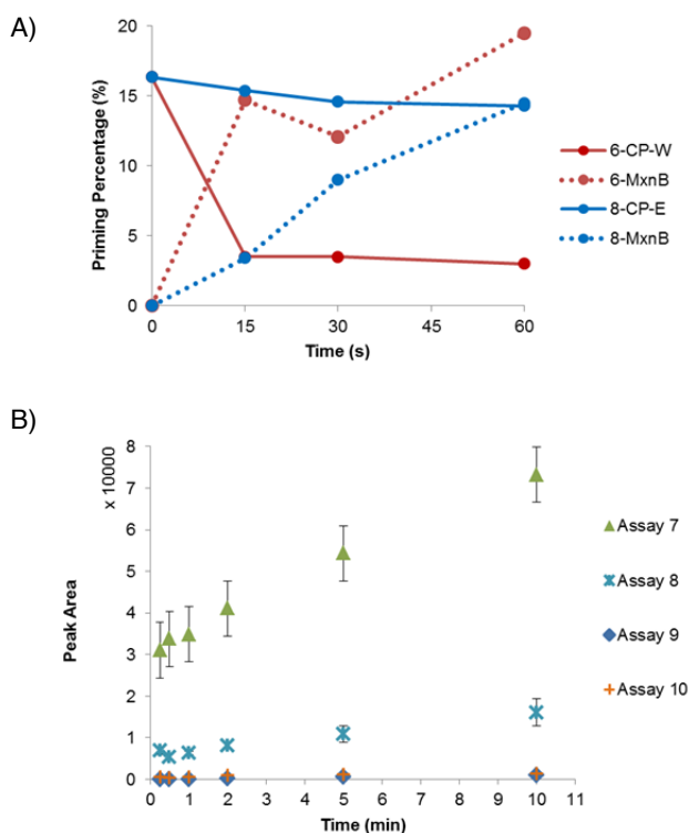
Fig. 4 LC-MS analysis of substrate transfer and competition assays. A) Percentage of primed MxnB and the remaining loaded-CP B) Time-course for the production of 9 from 15 s to 10 min. Peak area of extracted ion chromatograms for 8 were used for quantification. Assay 7-10: Assay 7 ( 6 -MxnB and 8 -CP-E), Assay 8 (MxnB, 6 -CP-W and 8 -CP-E), Assay 9 ( 8 -MxnB and 6 -CP-W), and Assay 10 (MxnB, 6 , and 8 ). Values for Assay 9 and 10 data points overlay. Error bars represent the standard error of the mean from three repeats.
