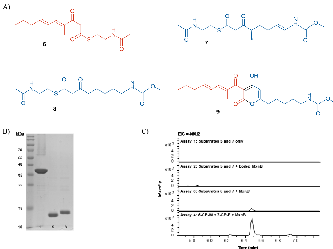
Fig. 2 Substrates and myxopyronin analogue, SDS Page and LC-MS Analysis of in vitro assays. A) SNAC substrates as native western mimic ( 6 ), native eastern mimic ( 7 ), analogue mimic of native eastern ( 8 ), and myxopyronin derivative ( 9 ). B) Lane 1: His-MxnB (38.7 kDa), lane 2: His-CP-E co-expressed with MtaA (14.7 kDa), and lane 3: His-CP-W co-expressed with MtaA (14.6 kDa) on a 15% SDS gel; C) LC-MS analysis of in vitro assays showing extracted ion chromatograms (EIC) [M+H]^+ = 406.2 : Assay 1 ( 6 and 8 only); Assay 2 ( 6 , 8 , and boiled MxnB); Assay 3 ( 6 , 8 , and MxnB); Assay 4 ( 6 -CP-W, 8 -CP-E, and MxnB).
