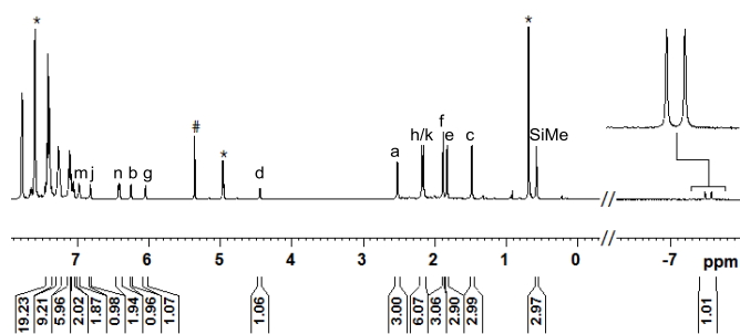
Fig. 1 ^1\text{H} NMR spectrum (500 MHz, \text{CD}_2\text{Cl}_2 , 300 K) of adduct 3ba , formed by reaction of complex 1b and hydrosilane 2a [ ^{\text{H}} = \text{CDCl}_3 , * = excess \text{MePh}_2\text{SiH} ( 2a )].
