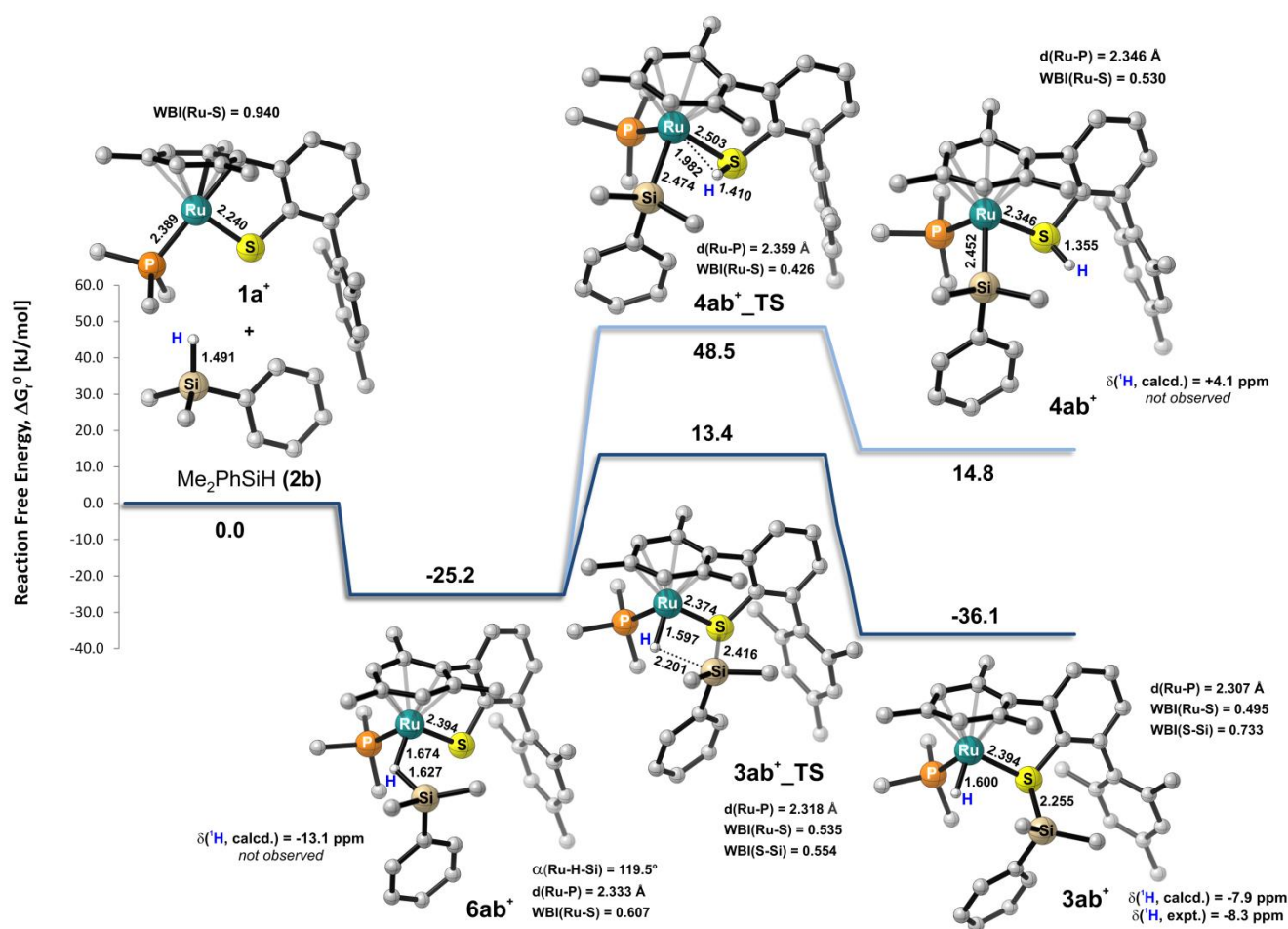
Fig. 5 Calculated relative free energies \Delta G_r^0 together with the structure of relevant intermediates and transition states for the Si–H bond activation of Me 2 PhSiH ( 2b ) by ruthenium(II) thiolate complex 1a + (results obtained at the B3LYP-D3(BJ)/ECP/6-31+G** level of theory using an SMD solvation model). All C–H hydrogen atoms are omitted for clarity. Bond lengths are in Å. Computed and experimental 1 H NMR shifts of intermediates are reported in ppm (with respect to TMS). Wiberg bond indices (WBI) of selected bonds are also indicated.
