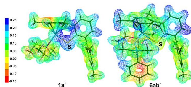
Fig. 7 Molecular electrostatic potentials (MEP) of [(Et_3P)Ru(SDmp)]^+ ( 1a + ) and [(Et_3P)Ru(SDmp)-Me_2PhSiH]^+ ( 6ab + ). Isovalue surfaces are displayed at an electron density of 0.04 a.u. (B3LYP/ECP/6-31+G** results). Red and blue regions correspond to the extreme negative and positive potentials, respectively.
