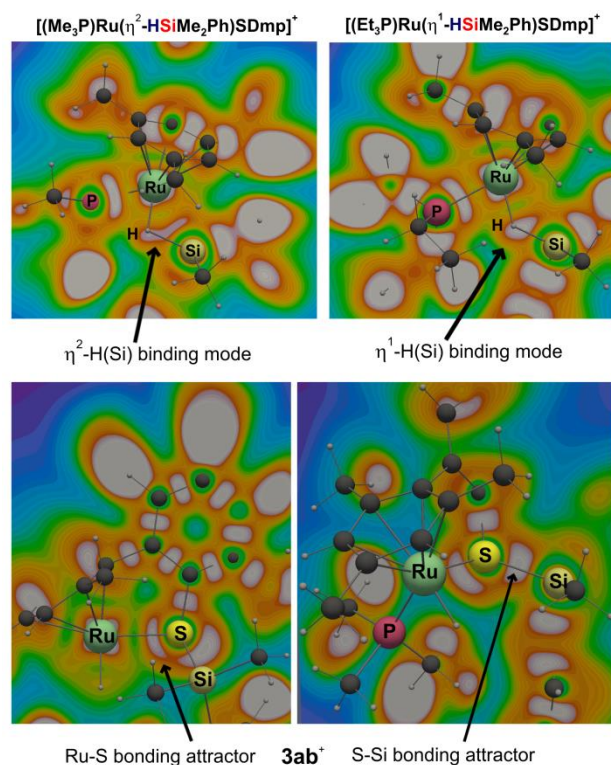
Fig. 6 Cut-plane plots from ELI-D analyses of bonding in hydrosilane complexes of [(R_3P)Ru(SDmp)]^+ ( R_3P = Me_3P , upper left and R_3P = Et_3P , upper right) with Me_2PhSiH ( 2b ), and in silylthioruthenium hydride intermediate 3ab + (lower). The gray-white regions represent ELI-D maxima (bonding attractors).
