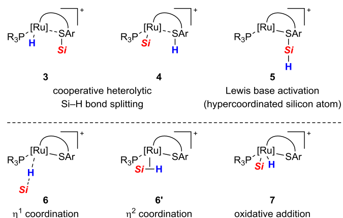
Chart 1 Possible modes for the Si–H bond activation by ruthenium(II) thiolate complexes 1 with (top) and without (bottom) participation of the sulfur atom.
