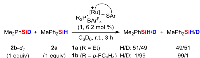
Scheme 5 1 H/ 2 H scrambling experiments: The crucial role of the phosphine ligand.
