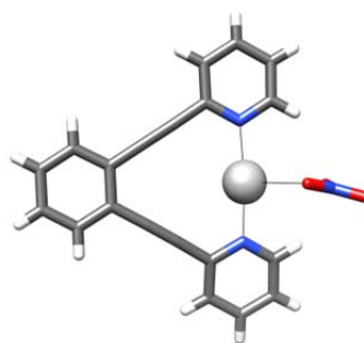
Fig. 8 The X-ray structure of 12-Ag .
