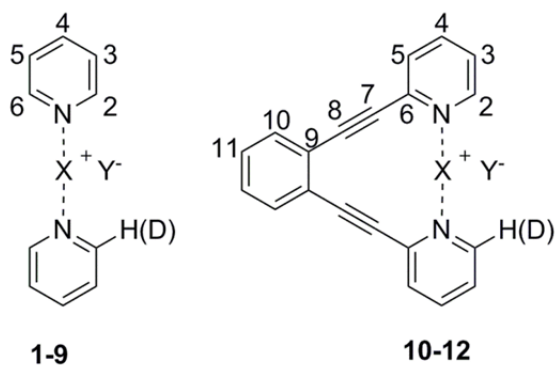
Fig. 1 The structure of the model systems assessed for elucidation of the counterion (Y - ) effect on the [N–I–N] + halogen bond (X = I): [bis(pyridine)iodine] + BF 4 - ( 1-I ), ClO 4 - ( 2-I ), PF 6 - ( 3-I ), SbF 6 - ( 4-I ), OTf ( 5-I ), TsO - ( 6-I ), NO 3 - ( 7-I ), and CF 3 CO 2 - ( 8-I ), and their geometrically restrained [(1,2-bis(pyridin-2-ylethynyl)benzene)iodine] + BF 4 - ( 10-I ), OTf ( 11-I ) and NO 3 - ( 12-I ) analogues. The BF 4 - of 9-I was scavenged with dodecabenzylbambus[6]uril (Bn 12 BU[6]). 47 The spectroscopic data of 1-I to 8-I was compared to those of the corresponding silver(I) complexes (X = Ag) 1-Ag to 8-Ag .
