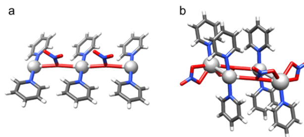
Fig. 7 X-ray crystallographic investigation of [\text{bis}(\text{pyridine})\text{iodine}]\text{nitrate} provided (a) pseudo-square planar N–Ag(NO 3 ) 2 –N ( 7-Ag ), and (b) coexisting pseudo-tetrahedral and pseudo-octahedral (5+1) N–(Ag)Ag(NO 3 ) 2 –N ( 7-Ag-2 ) coordination geometries.
