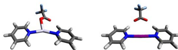
Fig. 5 The DFT-predicted equilibrium geometries of complexes 8-Ag and 8-I are shown to the left and right, respectively. Whereas silver(I) is predicted to form T-shaped, tris-coordinate species with a strongly bound counterion, short iodine-oxygen contact is not seen for the corresponding iodine(I) complex, which prefers a linear, bis-coordinate N–I–N geometry.
