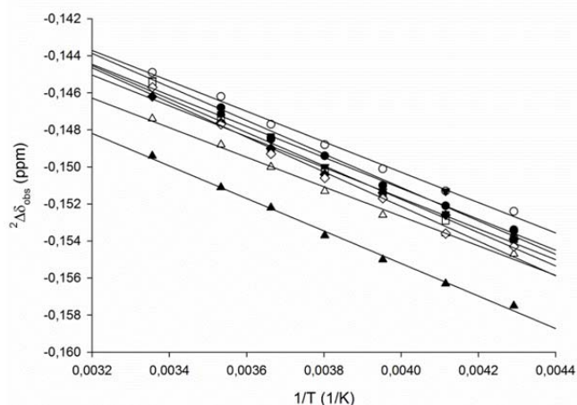
Fig. 4. The similar temperature dependence of the two-bond isotope effect ( {}^2\Delta_{\text{obs}} ) measured on C-3 of 1-I – 8-I indicates that the [\text{N}\cdots\text{I}\cdots\text{N}]^+ halogen bond is static, symmetric in solution, regardless of the counterion. \circ \text{BF}_4^- , \blacktriangledown \text{ClO}_4^- , \blacksquare \text{PF}_6^- , \square \text{SbF}_6^- , \bullet \text{OTf}^- , \blacklozenge \text{OTs}^- , \triangle \text{NO}_3^- , \blacktriangle \text{CF}_3\text{CO}_2^- , and \diamond \text{BF}_4^- .
