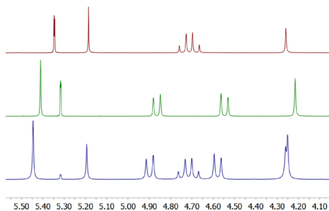
Fig. 3. The aliphatic region of the ^1\text{H} NMR of dodecabenzylbambus[6]juril ( \text{Bn}_{12}\text{BU}[6] ) in the absence and presence of complex 1/1-d . Top row (red) : The spectrum of free \text{Bn}_{12}\text{BU}[6] . Middle row (green) : the spectrum following addition of 1 eq. [bis(pyridine)iodine] ^+ tetrafluoroborate to the solution. The counterion is trapped as [(\text{Bn}_{12}\text{BU}[6])(\text{BF}_4^-)] . Bottom row (blue) : the spectrum of \text{Bn}_{12}\text{BU}[6] with 0.55 eq [bis(pyridine)iodine] ^+ tetrafluoroborate. Signals belonging to the \text{BF}_4^- complexed and the free \text{Bn}_{12}\text{BU}[6] are observed simultaneously, indicating strong \text{BF}_4^- binding. Hence, the use of an excess \text{Bn}_{12}\text{BU}[6] ensures the complete trapping of the anion from the dichloromethane solution.
