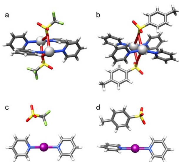
Fig. 6 The solid state geometries of complexes (a) 5-Ag , (b) 6-Ag , (c) 5-I and (d) 6-I obtained by X-ray crystallography reveal that the bis(pyridine) complexes of silver(I) form pseudo-tetracoordinated dimers, whereas those of iodine(I) form ionic, linear, bis-coordinated N–I–N complexes in the presence of moderately coordinating counterions, such as OTf − and OTs − .
