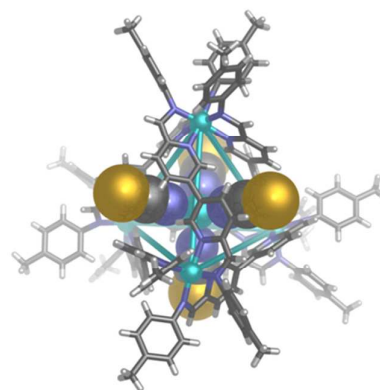
Fig 3: Visualisation of template anion – ligand proton orientation for [\text{Zn}(\text{NCS})_4]^{2-} \subset \text{Zn-1} and [\text{Zn}(\text{NCO})_4]^{2-} \subset \text{Zn-1} . Image based on the single crystal X-ray structure of [\text{CoBr}_4]^{2-} \subset \text{Co-1} , where the [\text{CoBr}_4]^{2-} guest is replaced with [\text{Zn}(\text{NCS})_4]^{2-} . Atom colours; carbon grey, hydrogen white, nitrogen blue, zinc(II) turquoise, sulfur gold.
