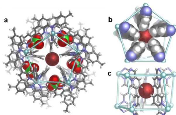
Fig 4: Single-crystal X-ray structure of \text{Br}^- \subset \text{Zn-2} ; a) indicating the overall connectivity of the structure; b) cut away view of the central binding pocket, highlighting the tight fit of the bromide anion within the central binding pocket; c) side on view of the same complex showing that the bromide anion is bound at the centre of the channel through H-bonding with ten inward-pointing pyridyl hydrogen atoms. Disorder is omitted for clarity.
