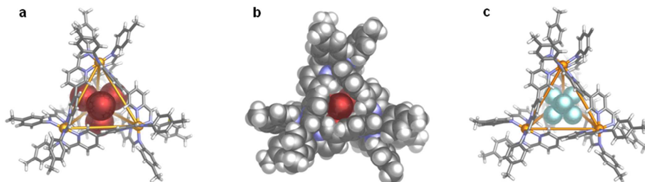
Fig 1: Single-crystal X-ray structures of \text{Co}_4\text{L}_6 tetrahedra; a) [\text{CoBr}_4]^{2-} \subset \text{1} , stick representation of the host with the centrally bound anion shown in a space-filling representation and b) host and guest both shown in space-filling mode, highlighting the tight fit of the guest within the symmetry-matched capsule; c) \text{SbF}_6^- \subset \text{Co-1} . Solvent, counterions and disorder are omitted for clarity. Atom colours; carbon grey, hydrogen white, nitrogen blue, cobalt(II) orange, bromine red, fluorine cyan.
