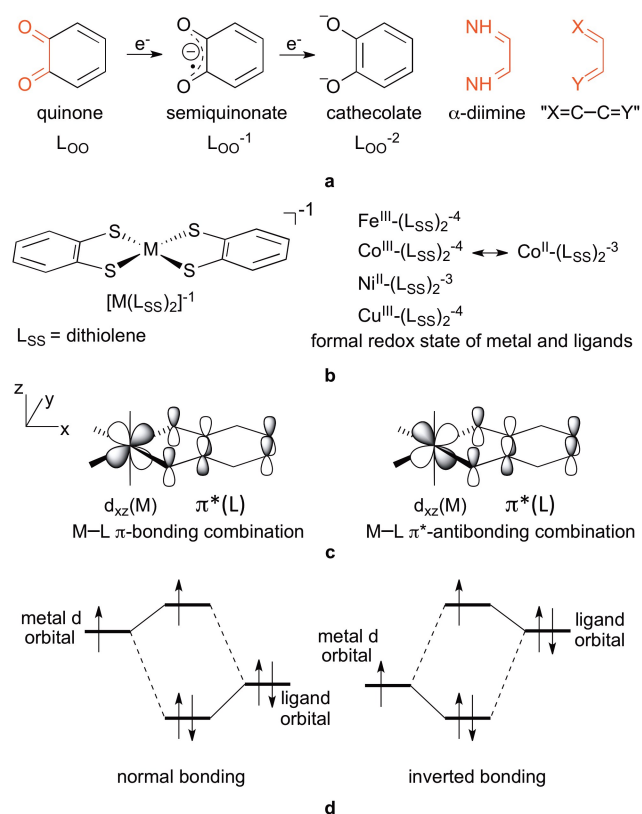
Figure 1. a Two-electron redox series of quinone to catecholate, \alpha -diimine, and the common X=C=C=Y structural motif, which also highlighted in red, b general structure of square-planar bis-dithiolenes complexes ( [M(L_{SS})_2]^{-1} ) and the assigned formal oxidation state of the metal and ligands for Fe, Co, Ni and Cu derivatives, c \pi -type interactions between the metal d-orbital ( d_{xz} ) and the redox-active orbital of quinoids, the magnitude of mixing of these metal- and ligand-based orbitals determines non-innocence, d normal and inverted bonding for a two-orbital-three-electron case, e.g. orbitals in c with three electrons.
