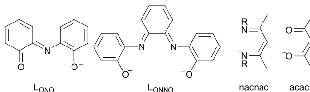
Figure 5. Arbitrary selection of redox active ligands, for which the same mechanisms presumably operate as for orthoquinoid derivatives.
