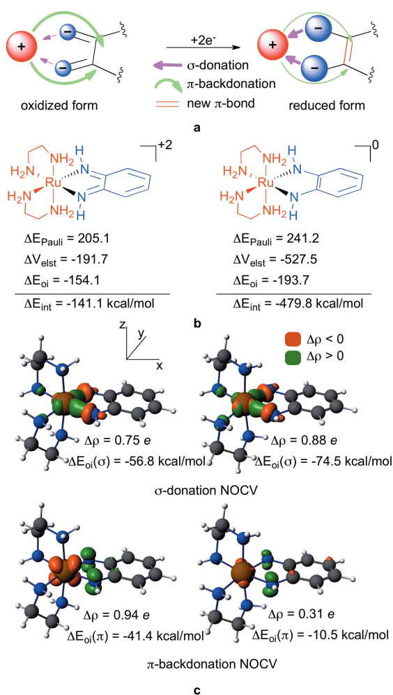
Figure 3. a. Explanation for the M–L interaction driven ligand reduction b. energy decomposition analysis for M–L interaction in [(en)_2RuL_{NN}]^{+2} (left) and [(en)_2RuL_{NN}]^0 (right), and c. NOCV orbitals representing \sigma -donations and \pi -backdonations for [(en)_2RuL_{NN}]^{+2} (left) and [(en)_2RuL_{NN}]^0 (right).
