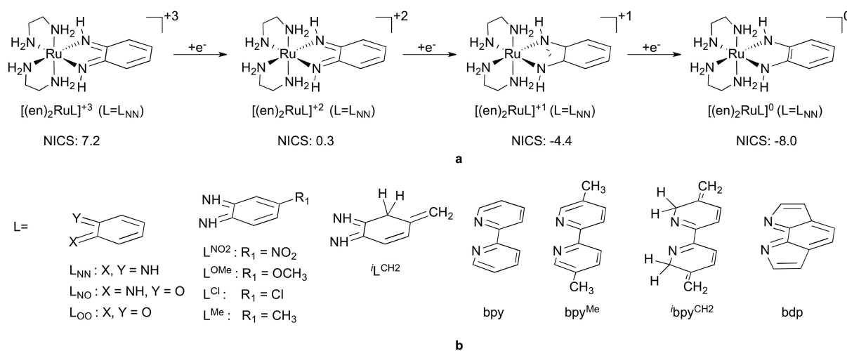
Figure 2. a . The four state redox series investigated for octahedral ruthenium complexes containing one non-innocent ligand, L, and two spectator 1,2-diaminoethane ( en ) ligands and NICS values computed for the six-membered carbon ring of L NN , b . redox active ligands investigated.
