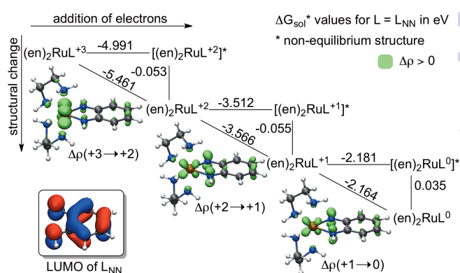
Figure 4. Theoretical square scheme for the [(en)_2RuL_{\text{NN}}]^{+3/+2/+1/0} redox series with the corresponding electron density change and the LUMO of L_{\text{NN}} .
