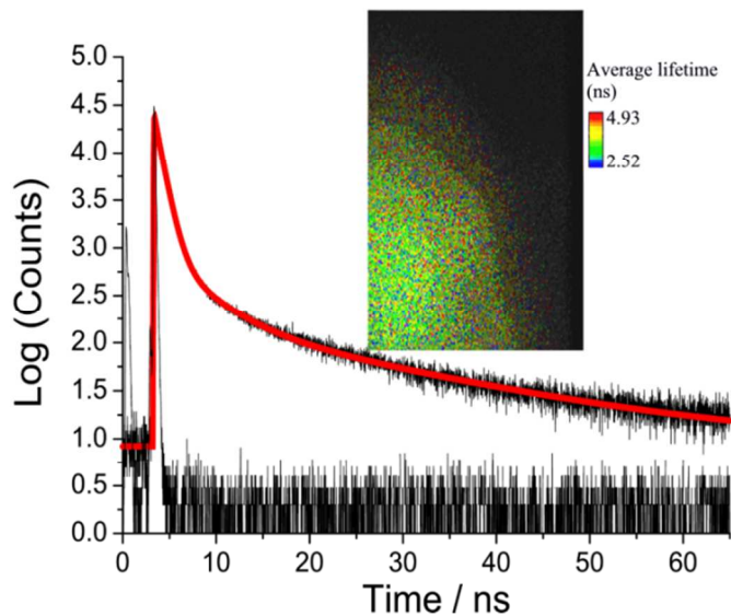
Figure 7. Room temperature emission decay curve and instrument response function recorded for O-DMIM and the least-squares fit to a tri-exponential (red line). Insert shows a typical fluorescence lifetime image taken for the crystal sample.
