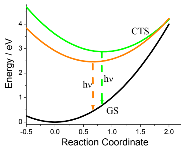
Figure 9. Constructed simplified potential energy surfaces diagram using determined parameters to show the difference between the emitting states for the two crystal forms. GS = ground state, CTS = charge transfer state.
