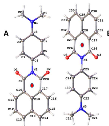
Figure 1. Molecular structure for O-DMIM showing the two related molecules in the unit cell. Note: red dots represent the centroids discussed in the main text.
