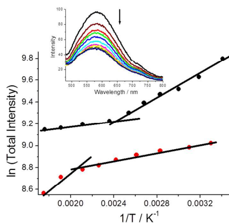
Figure 6. Plots to demonstrate the dependency of total fluorescence intensity versus 1/T ( \bullet = G-DMIM ; \bullet = O-DMIM ). Lines are drawn to help show the deviation points. Insert depicts fluorescence spectra for DMIM with increasing temperature.
