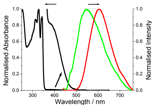
Figure 5. Room temperature absorption spectrum for DMIM in dilute cyclohexane and the expansion of the region around 400 nm. The fluorescence spectrum recorded for crystalline O-DMIM (red) and G-DMIM (green).
