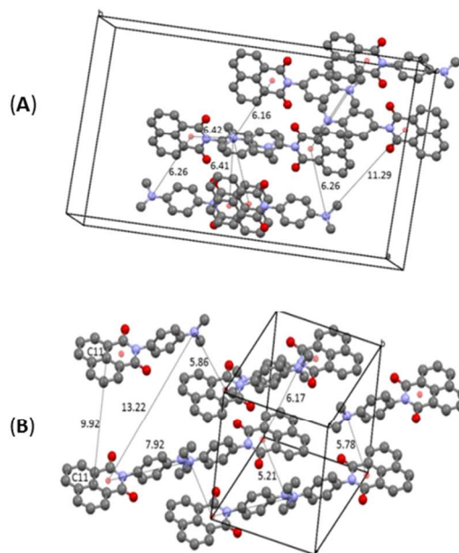
Figure 2. Selected crystal packing diagrams and intermolecular distances in Å for O-DMIM (A) and G-DMIM (B). Note: the 9.92 Å distance for structure B is the closest distance where the two naphthalimide units are parallel.
