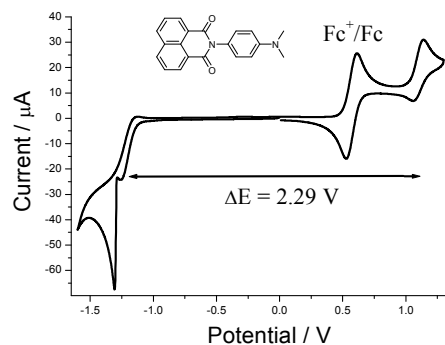
Figure 3. Cyclic voltammogram for DMIM in dry DCM (0.2 M TBATFB) at a glassy carbon working electrode vs Ag/AgCl. Scan rate = 50 mV s -1 .
