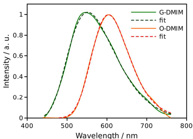
Figure 8. Fits of the emission spectra for G-DMIM and O-DMIM to a charge-transfer model. The measured spectra are shown by the solid lines and fits by the dashed lines.
