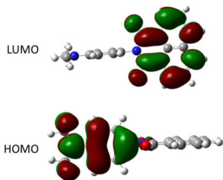
Figure 4. Representation of the HOMO and LUMO for DMIM calculated using DFT (B3LYP) and a 6-311G + (3df) basis set in a cyclohexane continuum solvent model.
