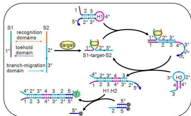
Fig. 1 Schematic diagram of the target-driven DNA association to cyclically mediate the assembly of hairpins system.
