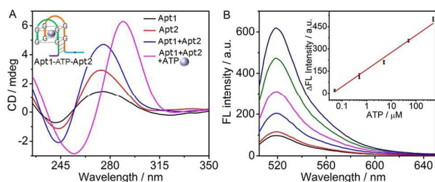
Fig. 3 (A) CD spectra of different solutions with the marked components at 5 \mu\text{M} Apt1 and Apt2, and 500 \mu\text{M} ATP. (B) Fluorescence spectra at 0, 0.05, 0.5, 5, 50, 500 \mu\text{M} ATP (from bottom to top). Insets: plot of \Delta F vs. logarithm of ATP concentration.
