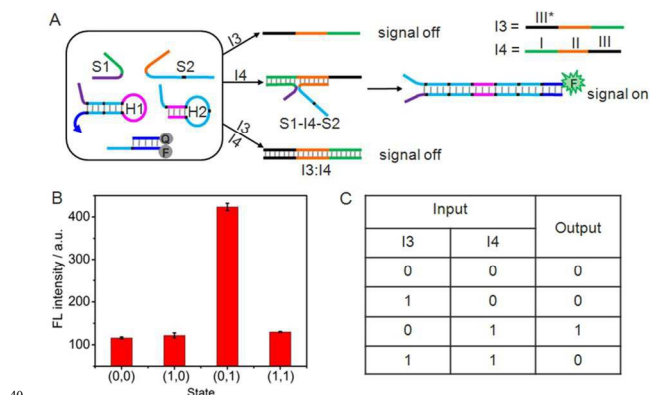
Fig. 5 (A) Illustration of the operational “INHIBIT” logic gate. (B) Fluorescence intensity measured at 520 nm. (C) Truth table of “INHIBIT” logic gate.
