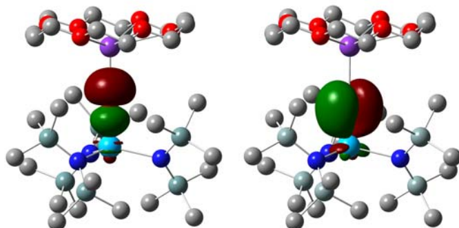
Fig. 4 One set of \sigma and \pi Th-N NLMOs in 6 . Hydrogen atoms omitted for clarity. Isosurface = 0.04.
