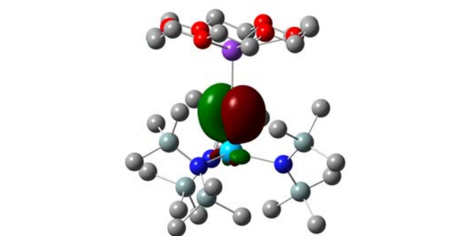
Fig. 3 \sigma and \pi Th-O NLMOs in 6 . Hydrogen atoms omitted for clarity. Isosurface = 0.04.
