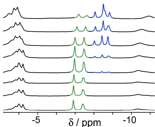
Figure 4. Series of 1 H NMR spectra (D 2 O, 298 K) of a mixture of cage (0.2 mM), C (0.2 mM) and B (2.0 mM). pH values (from bottom to top): 5.0, 7.4, 8.9, 9.6, 9.8, 10.6, 11.3, 12.2. Replacement of C (green signals) by B (blue signals) as the pH rises is clear.
