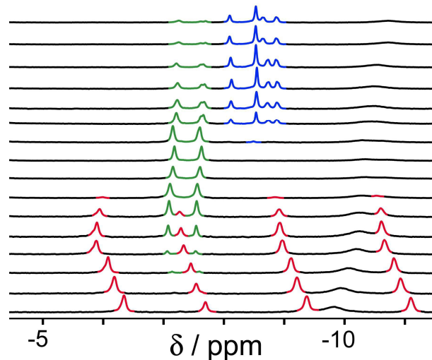
Figure 5. 1 H NMR spectra (D 2 O, 298 K) of a mixture of cage (0.2 mM), H 2 A (0.75 mM), B (7.1 mM) and C (0.2 mM), in the chemical shift region where the paramagnetically shifted signals from bound guests occur. pH values (from bottom to top): 2.0, 2.8, 4.3, 4.9, 5.7, 6.0, 6.5, 7.1, 8.1, 9.3, 9.7, 10.0, 10.6, 11.0, 11.5, 12.2. The change in occupancy of the cavity by the three different guests in succession is clear as the pH rises; the red, green and blue signals arise from the bound guests in the complexes cage • H 2 A , cage • C ; and cage • B (see Fig. 2).
