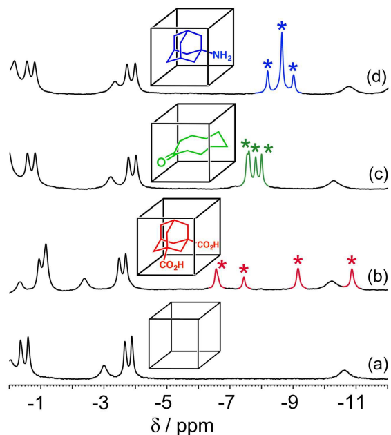
Figure 2. Parts of the 1 H NMR spectra ( \text{D}_2\text{O} , 298 K) of (a) free cage; (b) complex \text{cage}\cdot\text{H}_2\text{A} ; (c) complex \text{cage}\cdot\text{C} ; and (d) complex \text{cage}\cdot\text{B} , recorded at 0.2 mM cage in the presence of excess guest such that the cage was fully bound. This region of the NMR spectrum shows signals for the bound guests (highlighted), shifted by the paramagnetism of the host cage. The different spectroscopic signatures of each bound guest are distinct and clear in the region –6 to –10 ppm.
