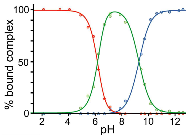
Figure 6. Graphical representation of the data obtained from the NMR spectra in Fig. 5, showing the proportion of each type of complex (red, cage • H 2 A ; green, cage • C ; blue, cage • B ), as a percentage of total complexed cage present, across the pH range. Dots represent measured data. The blue and red lines are calculated fits for pH-dependent binding of monobasic ( B ) and dibasic ( H 2 A ) guests, respectively (see ref. 14); the green line represents the calculated residual fraction of bound guest whose binding is not pH-dependent, i.e. cage • C .
