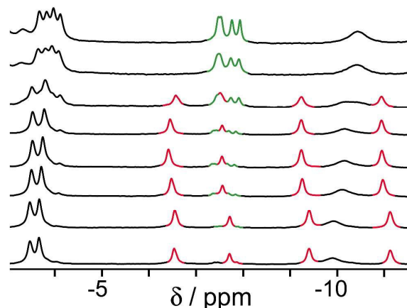
Figure 3. Series of 1 H NMR spectra ( \text{D}_2\text{O} , 298 K) of a mixture of cage (0.2 mM), C (0.2 mM) and \text{H}_2\text{A} (0.98 mM). pH values (from bottom to top): 2.0, 4.1, 4.3, 4.6, 5.0, 5.6, 7.3, 8.8. Replacement of \text{H}_2\text{A} (red signals) by C (green signals) as the pH rises is clear.
