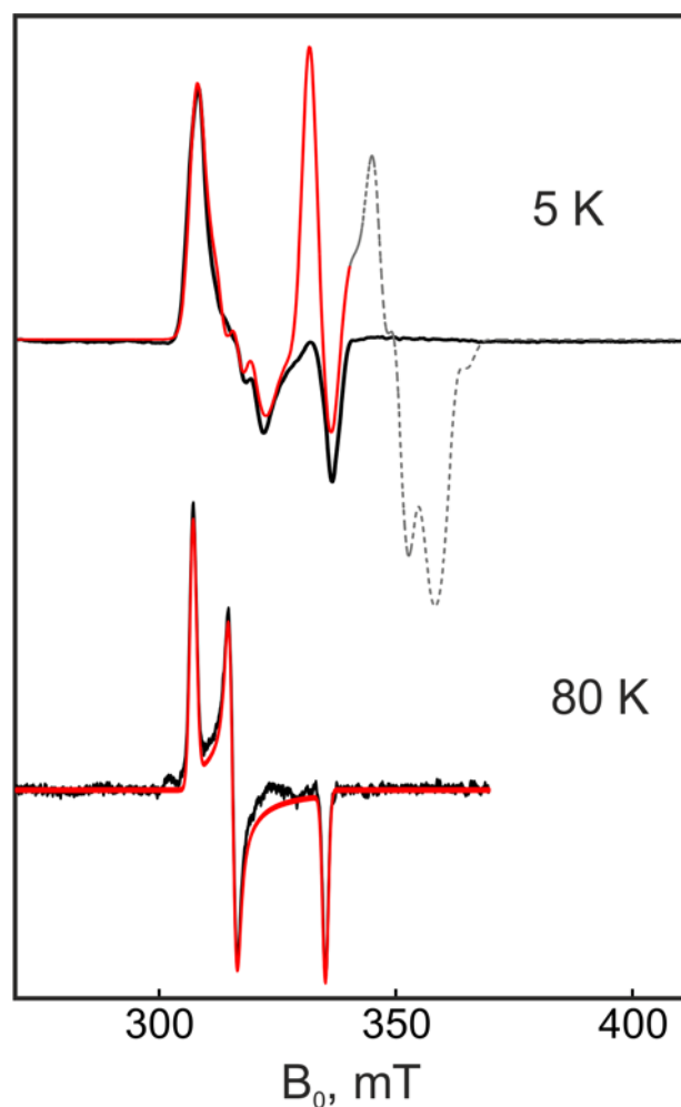
Figure 7. X-band CW EPR spectra of the dithionite-reduced \text{RH}_{\text{stop}} at two different temperatures, 5 K and 80 K, respectively. The experimental signals (black lines) and the simulations (red lines) correspond to the spin-coupled Ni-C sites since the contribution of the uncoupled Ni-C signal ('unsplit'), estimated to be < 30 % in the spectra, has been subtracted from the spectra. The part of the simulated spectrum that corresponds to the [\text{4Fe-4S}]^{1+} cluster signals is depicted with a dashed line (this was experimentally not detectable presumably due to g -strain effects and relaxation enhancement caused by spin-spin interactions). Because of the fast electronic relaxation of the FeS cluster signals at 80 K, their signals are not detectable and thus the 'fingerprint' of their magnetic interaction on the [\text{NiFe}] is absent from the NiC-related EPR signals. Experimental conditions: mw frequency 9.47 GHz, modulation amplitude 0.7 mT, mw power 0.2 mW.
