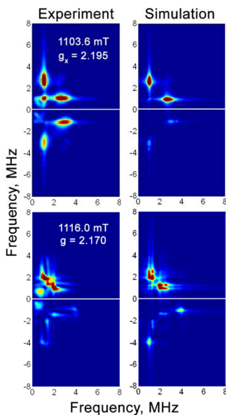
Figure 6 Q-band ^{57}\text{Fe} HYSCORE spectra of the \text{H}_2 -reduced forms of ^{57}\text{Fe} -enriched \text{RH}_{\text{stop}} at magnetic fields corresponding to two principal g -components of the Ni-C spectrum. Experimental conditions: mw frequency = 33.90 GHz, T = 20 K, \pi/2 = 40 ns, \tau = 300 ns, shot repetition time = 1 ms. Simulation parameters are given in Table 3.
