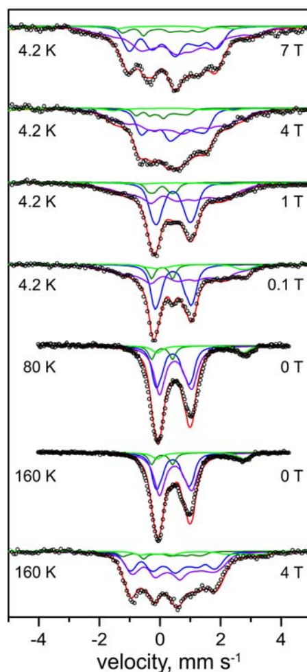
Figure 4. Mössbauer spectra of the H 2 -reduced form of 57 Fe-enriched R. eutropha RH stop . Parameters for the simulations and experimental conditions are listed in Table 2. The magnetic field (in Tesla) was applied perpendicular to the \gamma -beam. Open circles are the experimental data, solid lines represent the simulations: total (red line), [4Fe-4S] 2+ (blue line), [4Fe-4S] 1+ (purple line), low-spin Fe II (dark green line), N/O coordinated high-spin Fe II (light green line).
