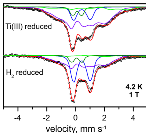
Figure 5. Mössbauer spectra of the Ti 3+ -citrate and the H 2 reduced forms of the RH stop recorded at 4.2 K and an external field of 1.0 T, applied perpendicular to the \gamma -beam. Parameters for the simulations and experimental conditions are listed in Table S3. Open circles are the experimental data, [4Fe-4S] 2+ (blue trace), [4Fe-4S] 1+ (purple trace), Fe II low spin of the [NiFe] site (green trace) and Fe II high spin (light green trace).
