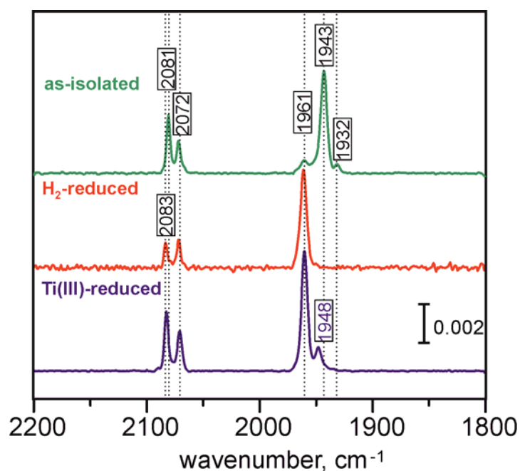
Figure 2. FTIR spectra of the RH from R. eutropha in its as-isolated (green trace), \text{H}_2 -reduced (red trace) and \text{Ti}^{3+} citrate-reduced (blue trace) states, which demonstrate the presence of 82% Ni-SI, 100% Ni-C and 85% Ni-C state, respectively. In the \text{Ti}^{3+} -citrate treated sample the band at 1948 \text{ cm}^{-1} , may be correlated with a substoichiometric accumulation of Ni-R, an assignment that is however precluded, because the expected bands of the corresponding CN ligands of Ni-R are absent. The absence of any additional Ni signals in EPR, suggest that the 1948 \text{ cm}^{-1} band corresponds either to a different conformation of Ni-C or to an EPR-silent state.
