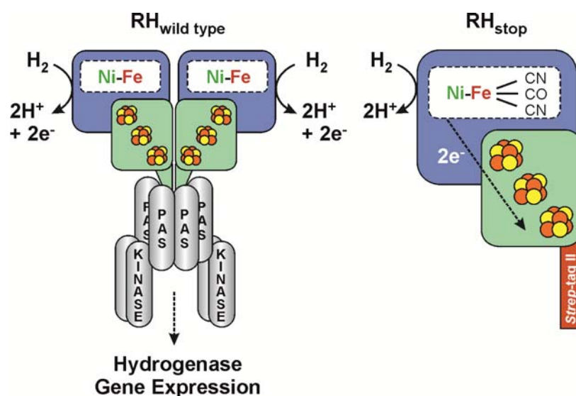
Figure 1. Scheme of the heterodimeric wild type RH hydrogenase in complex with the histidine kinase (left) and the RH stop derivative employed in this study (right). See also Ref. 36
