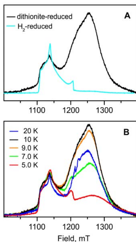
Figure 8. (A) Q-band field-swept 2-pulse echo-detected spectra of the H_2 -reduced (light blue trace) and sodium dithionite-reduced (black trace) forms of RH_{stop} (normalized to the Ni-C signal) recorded at 10 K. (B) Q-band field-swept 2-pulse echo-detected spectra of the sodium dithionite-reduced sample recorded at different temperatures. Experimental conditions: \tau = 300 ns, \pi/2 = 16 ns, shot repetition time = 20 ms ( H_2 -reduced). \tau = 300 ns, \pi/2 = 12 ns, shot repetition time = 20 ms (dithionite-reduced).
