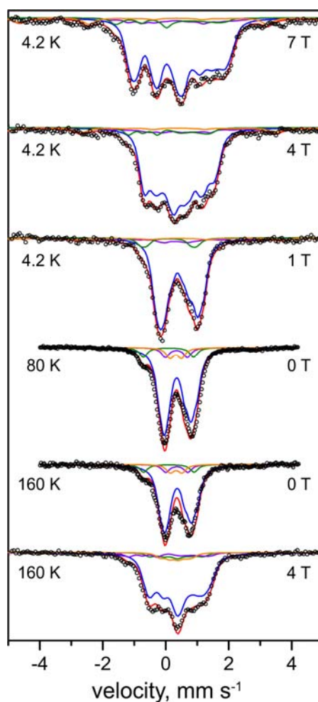
Figure 3. Mössbauer spectra of the as-purified form of 57 Fe-enriched R. eutropha RH stop . Parameters for the simulations and experimental conditions are listed in Table 1. The magnetic field (in Tesla) was applied perpendicular to the \gamma -beam. Open circles represent the experimental data, solid lines represent the simulations: [4Fe-4S] 2+ (blue line), [3Fe-4S] + (purple line), low-spin Fe II (green line), high-spin Fe III (orange line), total (red line).
