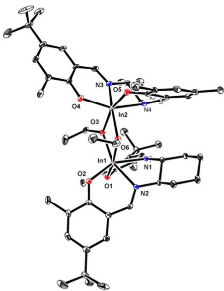
Figure 1. Molecular structure of (R,R) - 7 depicted with ellipsoids at 50% probability (H atoms and solvent molecules omitted for clarity).
