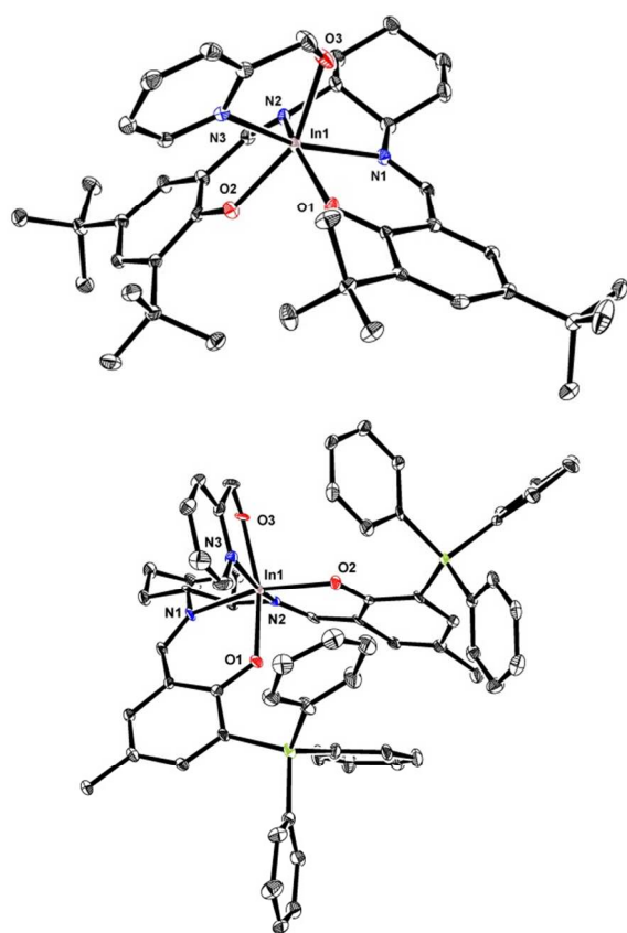
Figure 2. A (top) Molecular structure of (R,R) - 11 depicted with ellipsoids at 50% probability (H atoms and solvent molecules omitted for clarity) B (bottom) Molecular structure of (R,R) - 12 depicted with ellipsoids at 50% probability (H atoms omitted for clarity).
