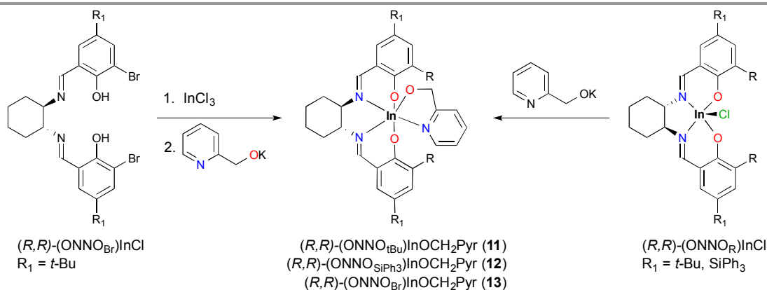
Scheme 3. Synthesis of (R,R)\text{-(ONNO}_R)\text{InOCH}_2\text{Pyr} complexes.
