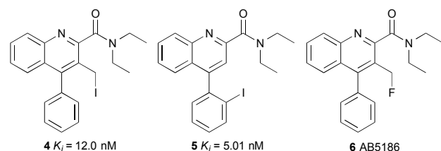
Figure 2. Quinoline-2-carboxamides 4 , 5 and 6 .
