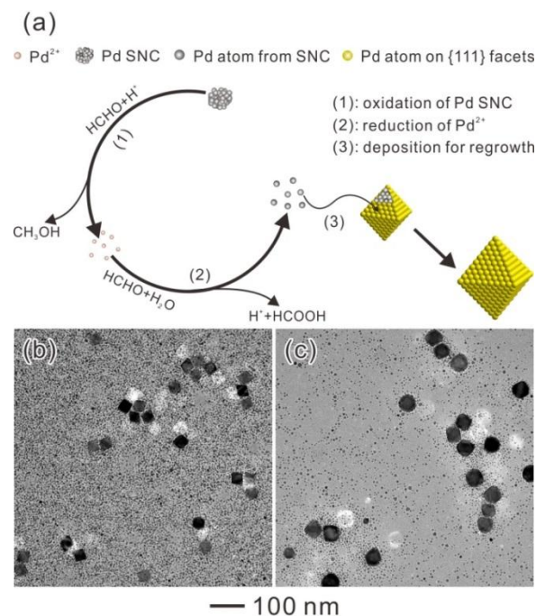
Fig. 4. (a) Schematic illustration of the three major steps involved in the oxidative etching and regrowth processes during Ostwald ripening. The redox reactions of HCHO enabled simultaneous reduction of \text{Pd}^{2+} and oxidation of \text{Pd}^0 . (b, c) TEM images of the products when the oxidation and reduction process was inhibited by adding extra (b) \text{HCOOH} , and (c) \text{CH}_3\text{OH} .
