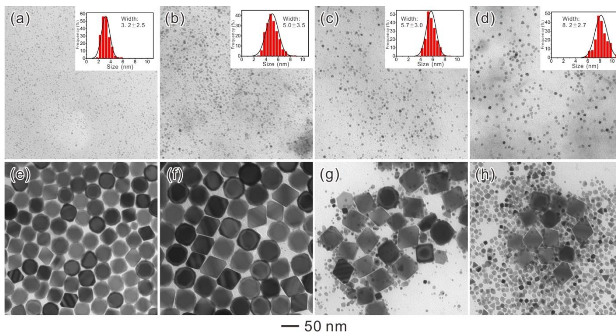
Fig. 6. (a-d) TEM images of four SNC samples with different particle sizes obtained by controlling the amount of \text{Na}_2\text{PdCl}_4 in the reaction: (a) 14.5 mg, (b) 29 mg, (c) 57 mg, and (d) 114 mg. The inset in each panel shows the size distribution of SNCs. (e-f) Corresponding products after 3 days of ripening.
