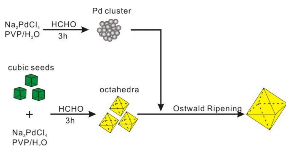
Fig. 1. Schematic illustration of Ostwald ripening in bimodal-sized Pd colloidal system.
