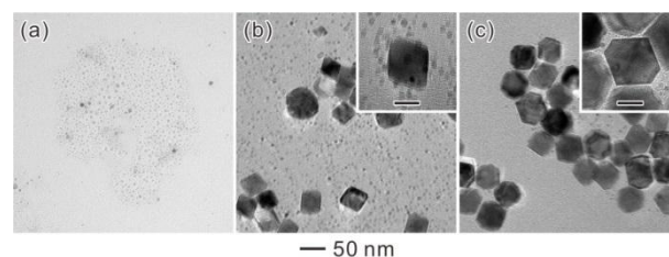
Fig. 5. TEM images of Pd (a) SNCs and (b) final products obtained by using the standard process except for substituting HCHO with AA as the reducing agent. The ripening can be recovered by the additional 100 μl HCHO (c). The inset shows the TEM image of Pd nanocrystals of (b) and (c) at a higher magnification (scale bars: 20 nm).
