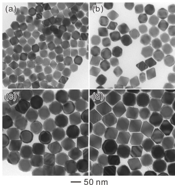
Fig. 9. TEM images of Pd octahedra with different edge lengths that were prepared using the standard procedure except different concentrations of Pd seeds: a) 4.2 \mu\text{M} , b) 3.1 \mu\text{M} , c) 1.0 \mu\text{M} , and d) 0.4 \mu\text{M} respectively.
