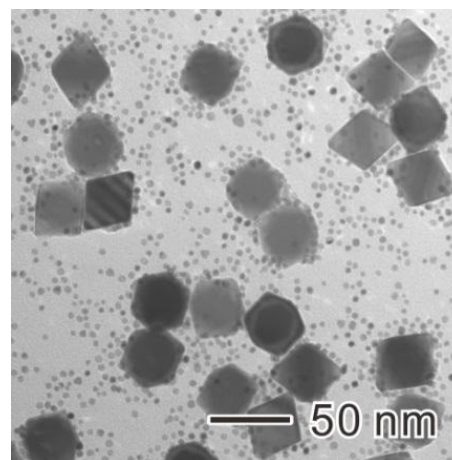
Fig. 7. TEM image of Pd nanocrystals prepared with 57.0 mg of \text{Na}_2\text{PdCl}_4 . In addition to Pd octahedrons of 37 nm in edge length, small Pd nanoparticles of 3 nm in size also formed. In this case, simply increasing the amount of Pd precursor did not increase the size of large Pd octahedrons.
