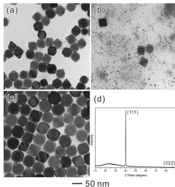
Fig. 2. (a-c) TEM images of (a) octahedral seeds, (b) mixture of seeds with SNCs ( t = 0 s), (c) the system after self-focusing process ( t = 72 h). (d) XRD pattern of the sample in (c).
