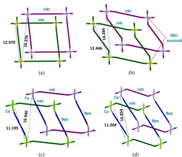
Fig. 5. Schematic representation showing extent of bending and internodal distances for ndc and bpy; (a,b) 2fa and 2fa' viewed perpendicular to bpy, respectively and (c,d) 2fa and 2fa' viewed perpendicular to ndc, respectively.
