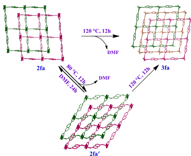
Scheme 1. Schematic representation showing bending and switching of interpenetration in the [\text{Co}_2(\text{ndc})_2(\text{bpy})] system.
