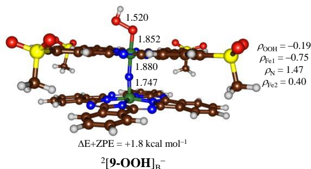
Fig. 7. DFT optimized geometries of ^2[9\text{-OOH}] at the B3LYP level of theory. Bond lengths are in angstroms and spin densities ( \rho ) in atomic units.
