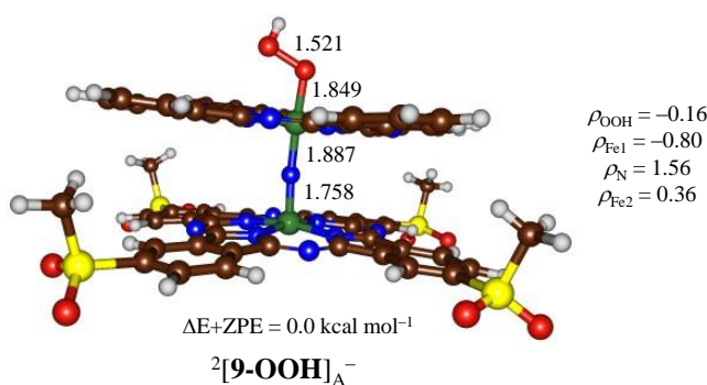
Fig. 6. DFT optimized geometries of 9 at the B3LYP (BP86) level of theory. Bond lengths are in angstroms and spin densities ( \rho ) in atomic units.
