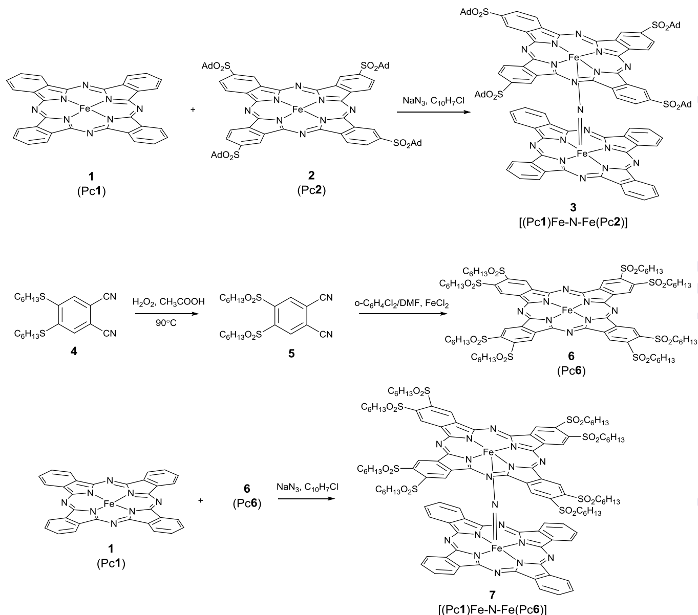
Scheme 2. Preparation of heteroleptic \mu -nitrido alkyldisulfonyl phthalocyaninato iron(II) 3 and 7 .
