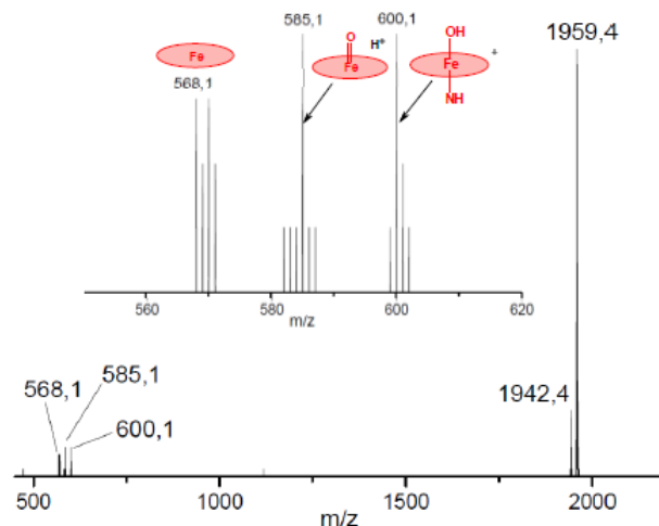
Fig 5. CID MS/MS spectrum of the oxo complex obtained from [(Pc2)FeNFe(Pc1)] and m -CPBA. An enlarged region of the spectrum with assignment of fragments is shown in the inset.
