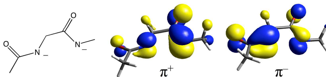
Figure 8. The diamidate moiety in NHase (left) and its in-phase (center) and out-of-phase (right) \pi MO combinations.
