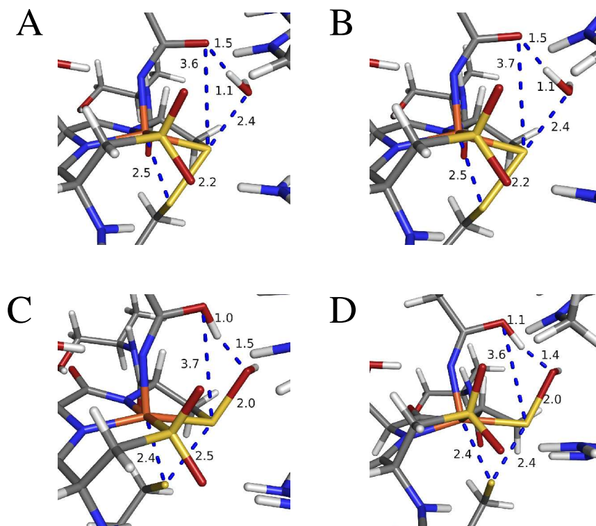
Figure 19. Structures of (A) Linear transit species with a water O – cyclic intermediate S distance of 2.4 Å, (B) IRC step towards reactants with this same distance, (C) SOH species, and (D) IRC step towards products. All distances are in Å.
