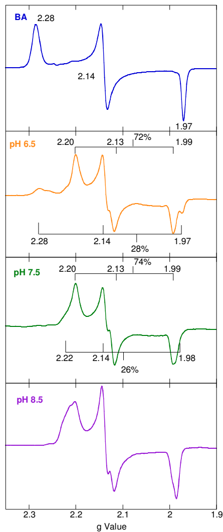
Figure 5. 77 K X band EPR Spectra of NHaseBA (blue) and NHaseAq at pH 6.5 (orange), 7.5 (green) and 8.5 (purple).
