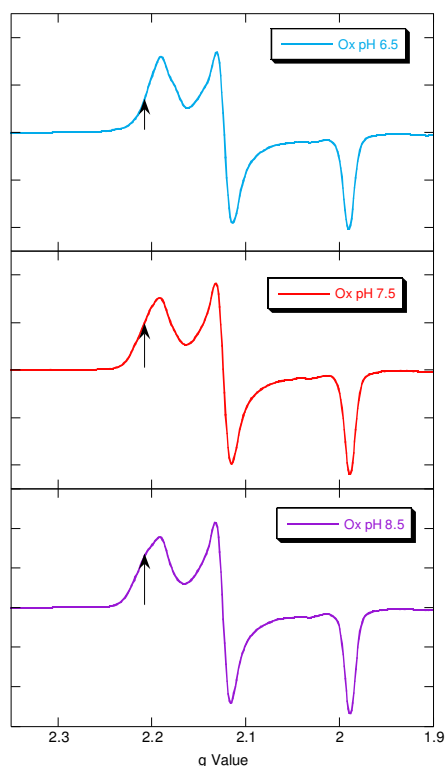
Figure 6. 77 K X Band EPR Spectra of NHaseOx at pH 6.5 (cyan), 7.5 (red), and 8.5 (purple). Signals from minor species at low field marked with arrows.
