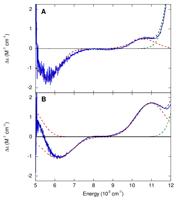
Figure 7. NIR MCD of NHase. 1.5 K, 7 T NIR MCD spectra of NHaseBA (A) and NHaseAq (B) at pD 7.5. Experimental data are in blue, the fit is in black dashes, red dashed curves denote d-d transitions and the green dashed curve denotes the thiolate-to- d\pi LMCT.
