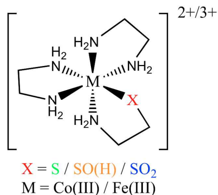
Figure 4. General structure of the [(en) 2 CMXCH 2 CH 2 NH 2 )-N,S] 2+/3+ complexes.
