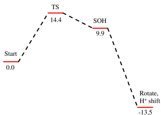
Figure 18. Reaction coordinate for nucleophilic attack by water on the S atom of the cyclic structure. Species defined at bottom of Figure 17, with zero energy referenced to the cyclic intermediate at -0/9 kcal/mol in Figure 16. All energies are given in kcal/mol.
