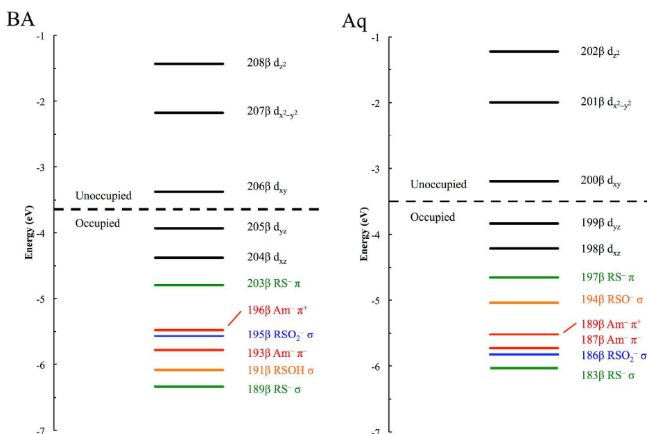
Figure 13. \beta MO Energy Diagram for NHaseBA (left) and NHaseAq (right). Metal d MOs are in black, thiolate MOs in green, sulfinate MOs in blue, sulfenate MOs in orange, and amidate MOs in red.
