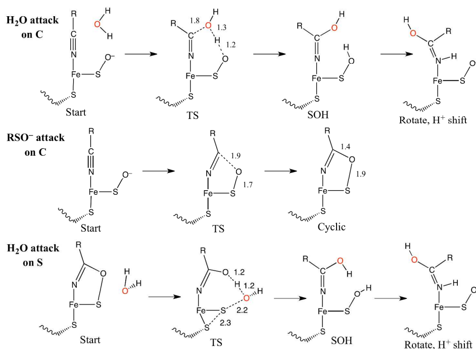
Figure 17. Structures listed for the reaction coordinates of Figures 16 and 18. All distances are in Å.
