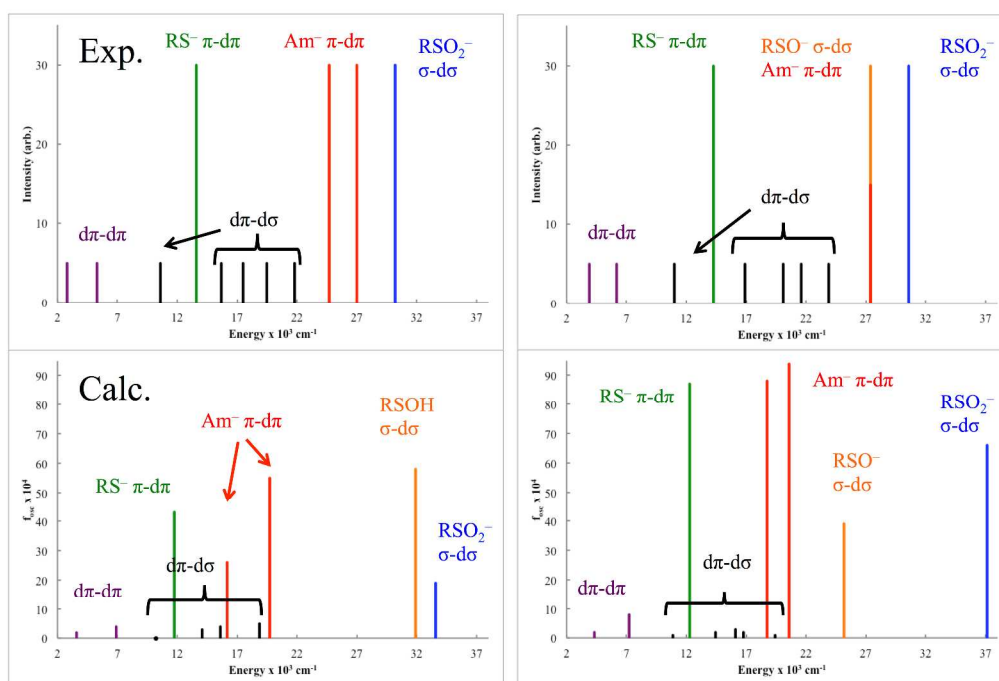
Figure 15. Experimental (top) and TD-DFT (bottom) transitions for NHaseBA (left) and NHaseAq (right). Lines are colored purple for d\pi \rightarrow d\pi , black for d\pi \rightarrow d\sigma , green for Cys- S^- \pi \rightarrow d\pi , red for amidate \pi \rightarrow d\pi , orange for Cys-SOH/ -SO^- \sigma \rightarrow d\sigma and blue for Cys- SO_2^- \sigma \rightarrow d\sigma . The transition at \approx 27000 \text{ cm}^{-1} in the upper-right plot is marked half red, half orange to denote the overlap of the amidate d\pi \rightarrow d\pi and Cys- SO^- \sigma \rightarrow d\sigma transitions.
