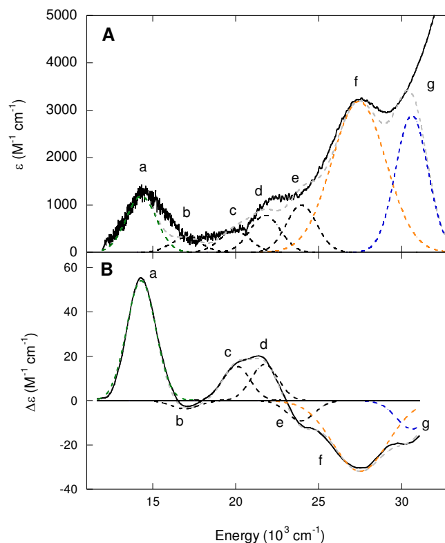
Figure 11. UV-Vis spectra of NHaseAq. (A) Absorption spectrum of NHaseAq at 5 K. (B) 5 K 7 T MCD spectrum of NHaseAq. Experimental data are in black, the total fit is in dashed gray, and dashed Gaussian curves denote Cys-S - \pi \rightarrow d\pi (a, green), d\pi \rightarrow d\sigma (b-e, black), Amidate \pi \rightarrow d\pi / Cys-SO - \sigma \rightarrow d\sigma (f, orange) and Cys-SO 2 - \sigma \rightarrow d\sigma (g, blue) transitions.
