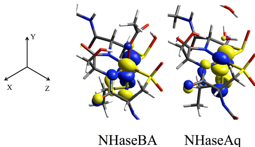
Figure 14. NHase \beta LUMOs. Isosurface contour plots of the DFT-calculated, d_{xy} \beta MOs of NHaseBA (center) and NHaseAq (right), along with the coordinate system for both models (left).
