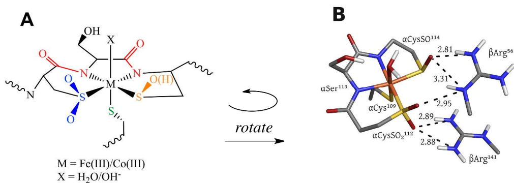
Figure 1. The active site structure of NHase. (A) Diagram of the NHase active site, depicting the thiolate (green), amidate (red), sulfinate (blue), sulfenate/sulfenic acid (orange) and water-derived (denoted X) ligands. (B) The Fe(III) active site of Rhodococcus erythropolis N771 NHase after photolysis (PDB ID 2CYZ). Heavy atom distances showing H bonding are marked with dashed lines. All distances are in Å.
