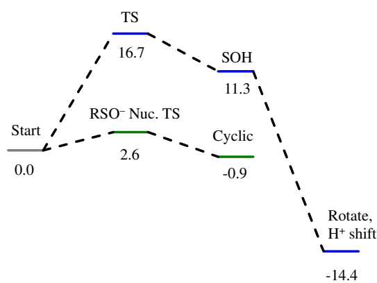
Figure 16. Reaction coordinates for attack on coordinated nitrile by water (blue) and attack on coordinated nitrile by sulfenate (green). All energies are in kcal/mol.
