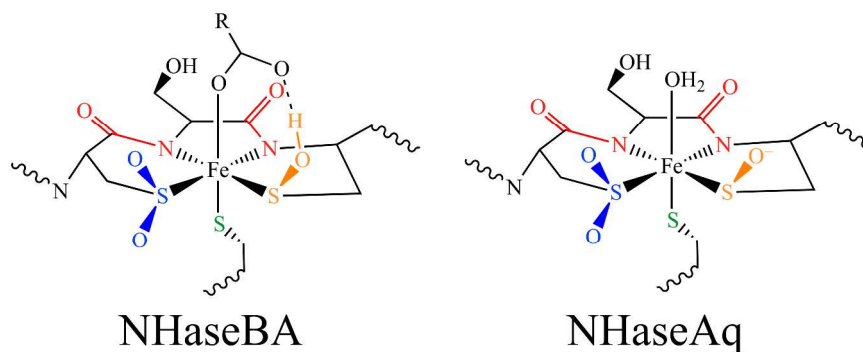
Figure 20. Spectroscopically determined active site structures of NHaseBA (left) and NHaseAq (right).
