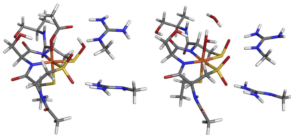
Figure 12. Geometry-optimized structures of NHaseBA (left) and NHaseAq (right).
