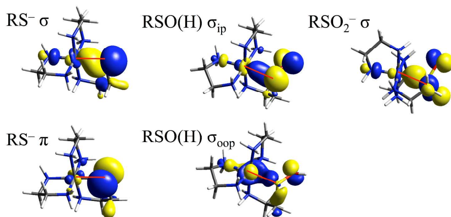
Figure 9. Molecular orbitals of thiolate, sulfenate, and sulfinate ligands involved in model complex LMCT transitions. Red lines mark the Fe-S bond in each picture.
