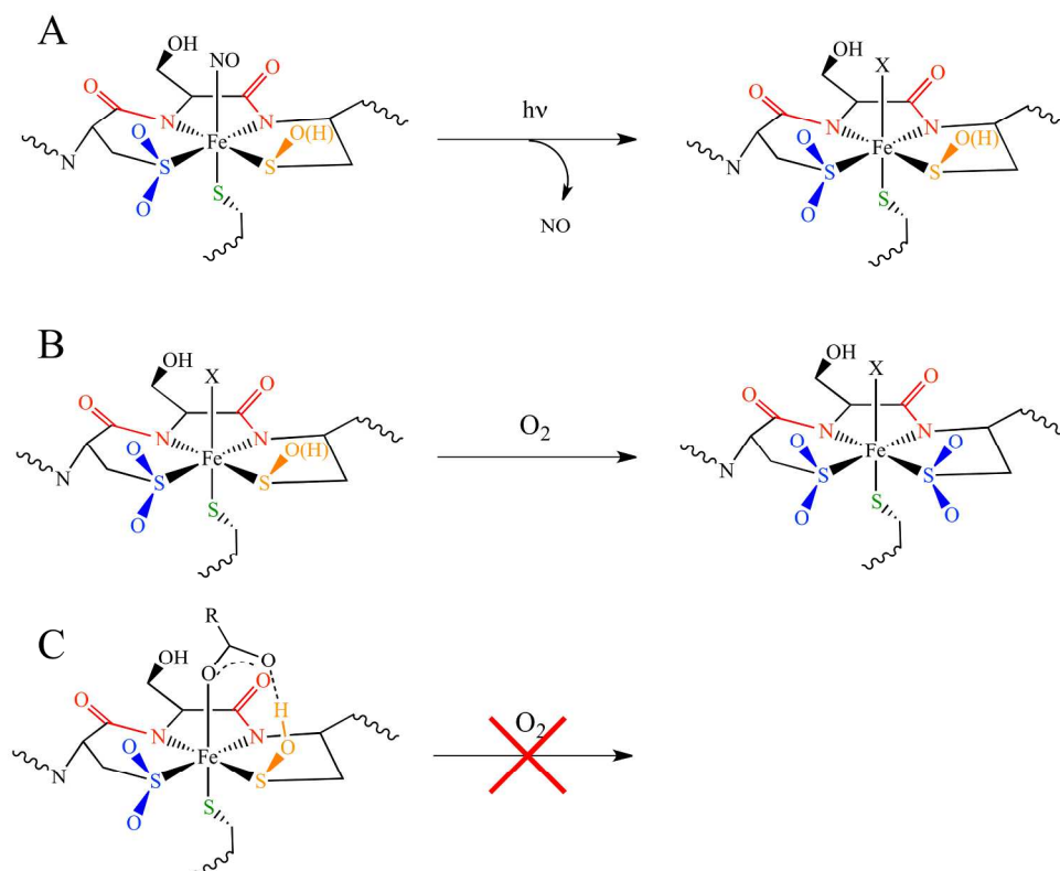
Figure 2. NHase active site forms. (A) Photolytic cleavage of Fe-bound NO to produce the active form. (B) Oxidation of the active form sulfenate/sulfenic acid group in aerobic conditions. (C) Protection of the active site through complexation with butyrate.
