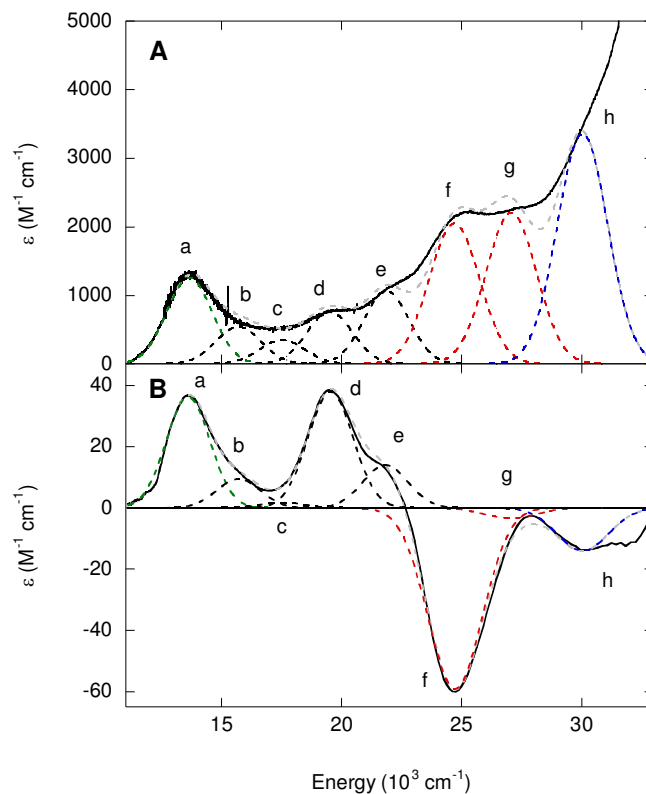
Figure 10. UV-Vis spectra of NHaseBA. (A) Absorption spectrum of NHaseBA at 5 K. (B) 5 K 7 T MCD spectrum of NHase BA. Experimental data are in black, the total fit is in dashed gray, and dashed Gaussian curves denote Cys-S - \pi \rightarrow d\pi (a, green), d\pi \rightarrow d\sigma (b-e, black), Amidate \pi \rightarrow d\pi (f-g, red) and Cys-SO 2 - \sigma \rightarrow d\sigma (h, blue) transitions.
