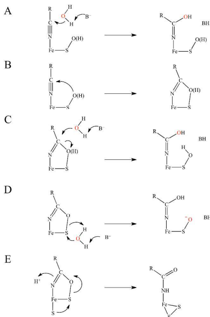
Figure 3. Potential mechanisms for NHase catalysis. (A) Activation of coordinated nitrile for nucleophilic attack by water. (B) Nucleophilic attack by RSO(H) and subsequent activation for attack by water on either (C) the nitrile carbon, or (D) the RSO(H) sulfur. The oxygen atom originating from water is shown in red. (E) Nucleophilic attack on the cyclic intermediate by the axial thiolate.
