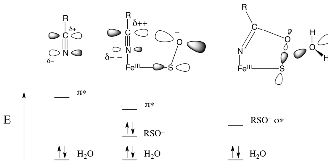
Figure 21. Donor/acceptor orbitals for free nitrile and water (left), coordinated nitrile and water (center) and the coordinated cyclic species and water (right).
