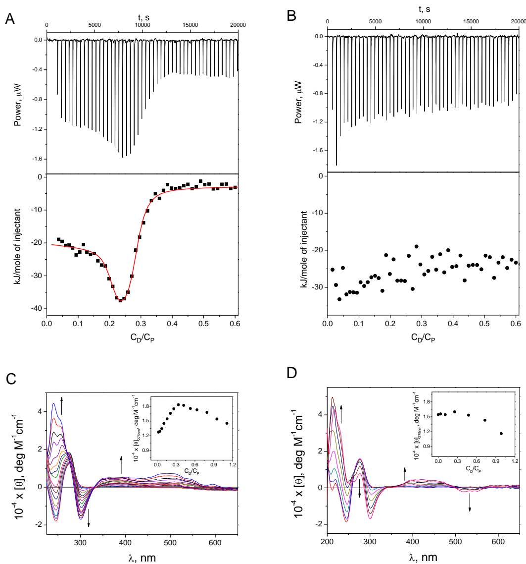
Fig. 2 Ag-AQCs clusters prevent the binding of DOX to ct-DNA. ITC profile obtained for (A) DOX/(ct-DNA+Ag + ) system, and (B) DOX/(ct-DNA +Ag-AQCs) system, C_P = 400 \mu\text{M} . CD spectra recorded for (C) DOX/(ct-DNA+Ag + ) system, and (D) DOX/(ct-DNA+Ag-AQCs) system. Inset: Molar ellipticity versus C_D/C_P ratio at \lambda = 275 \text{ nm} , C_P = 50 \mu\text{M} , ionic strength = 2.5 mM, pH = 7 and T = 25^\circ\text{C} .
