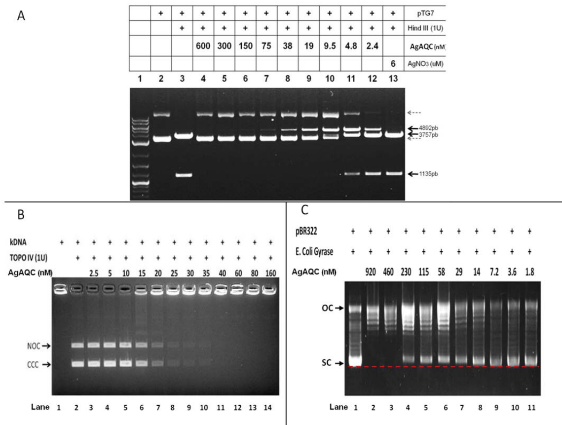
Fig. 3 Agarose gel electrophoresis showing the inhibition by Ag-AQCs of A) restriction enzyme HindIII activity. The pTG7 plasmid (lane 2) was incubated for 30 min at 37°C with one HindIII unit (lane 3) in the presence of nanomolar concentration of Ag-AQCs (lanes 4-12), or AgNO 3 (6 uM, lane 13), the reaction products were run on agarose gel. Continuous arrows indicate the theoretical products obtained after cut of the plasmid. Dotted arrows indicate the location of the plasmid with different supercoiling conformations. Lane 1, molecular weight markers. B) E. coli Topoisomerase IV decatenation activity. This gel contains ethidium bromide, which allows one to clearly resolve Topoisomerase IV generated nicked (NOC) and covalently closed circular (CCC) DNA. The kDNA networks are too large to enter the gel; C) E. coli DNA gyrase activity. The open-circular (OC) and supercoiled (SC) DNA are resolved and the relaxed DNA species are present as a Gaussian distribution of topoisomers, SC DNA has less mobility with increasing Ag-AQCs concentrations (dotted red line, lanes 4-9). The images are representative of at least three independent experiments.
