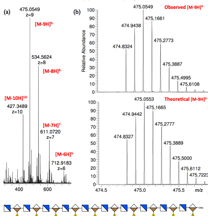
Fig. 7: Nano-electrospray mass spectral data for icosasaccharide [GlcNH 2 -IdoA2S] 10 -OMe 18 . (a). Main ions observed for z=7 (27%), 8 (72%), 9 (100%) and 10 (41%). (b). Observed and theoretical isotope patterns for major ion [M-9H] 9- . (LTQ Orbitrap XL)
