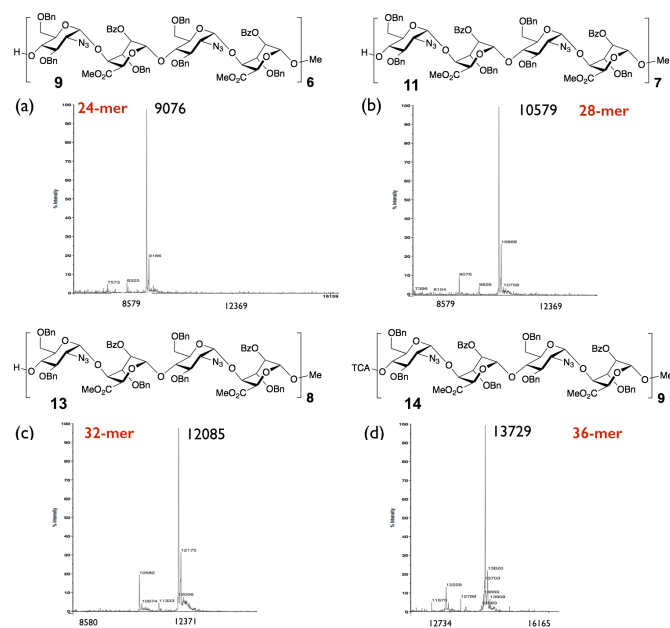
Figure 3: MALDI mass spectra of protected long oligosaccharides. (a) 24-mer, 9 . (b) 28-mer, 11 . (c) 32-mer, 13 . (d) 36-mer, 14 .
