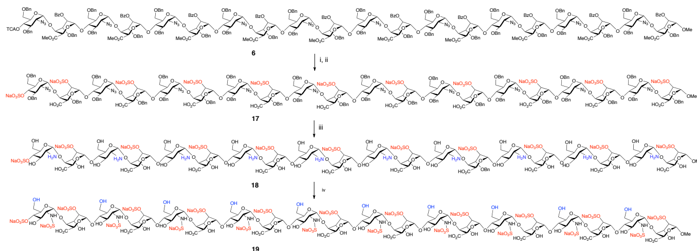
Fig. 6: Deprotection and sulfation to afford homogeneous heparin-like 20-mers [GlcNH 2 -IdoA2S] 10 -OMe, 18 and [Glc6SNS-IdoA2S] 10 -OMe, 19 . i) LiOH, THF/MeOH/H 2 O, 48%. ii) NMe 3 SO 3 , DMF, μW, 44 90%. iii) Pd(OH) 2 /C, EtOH/H 2 O, H 2 , 89%. iv) PyridineSO 3 complex, H 2 O.
