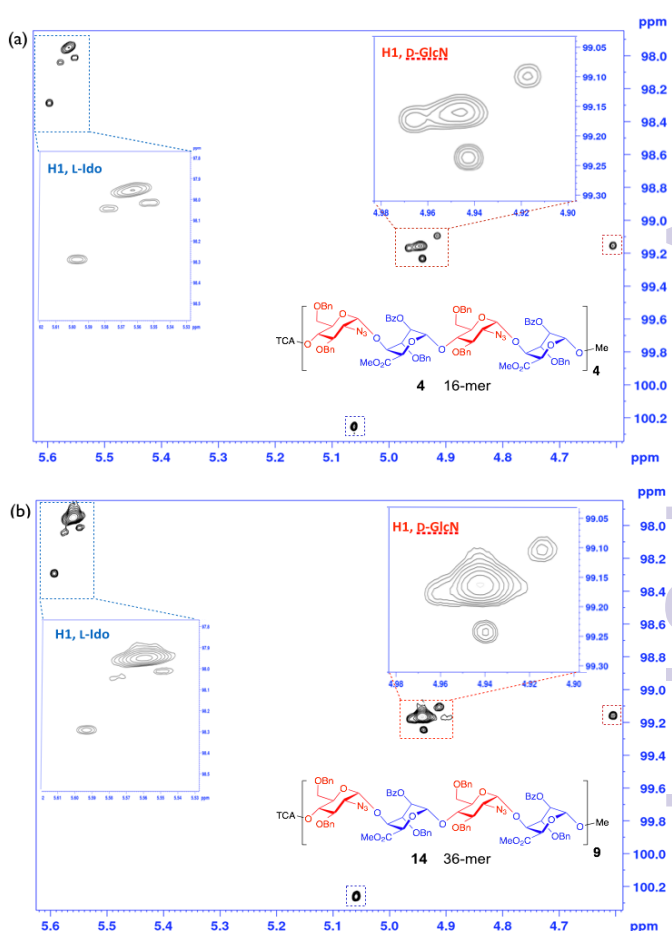
Fig. 5: NUS Pure Shift HSQC 800MHz data for long oligosaccharides: (a). 16-mer, 4 . (b). 36-mer, 14 . Inset expansions.
