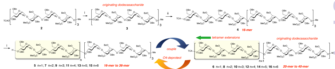
Fig. 2: Elongation from 12-mer 3 through to 40-mer 15 . i) MeOH, Pyridine, ii) NIS, AgOTf (cat.), DCM, 1 , n=1: 4 , 76%, 5 , 90%; n=2: 6 , 81%, 7 , 97%; n=3: 8 , 77%; 9 , 95%; n=4: 10 , 75 %, 11 , 93%; n=5: 12 , 78%; 13 , 93%; n=6: 14 , 72%, 15 , 87%; 16 , 64%, n=7.
